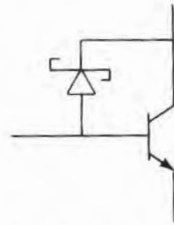
(a) Schottky clamped silicon transistor
