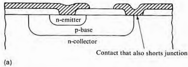
FIGURE 11.31 Effect of a shorted collector-base junction on emitter-base current.
