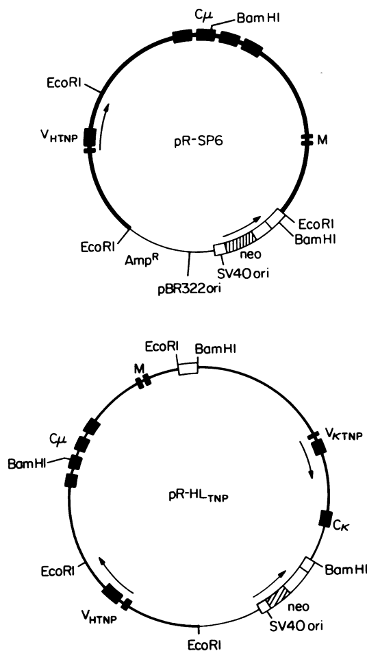
FIG. 1. Structure of the pR-Sp6 and pR-HL TNP plasmids. pR-Sp6 contains the functionally rearranged \mu_{\text{TNP}} gene ( \approx 16 kbp), which was inserted into the EcoRI site of pSV2- neo (see text). In addition to the \mu_{\text{TNP}} gene, pRHL TNP contains the functionally rearranged \kappa_{\text{TNP}} gene (9.6 kbp) at the BamHI site (2). Ig genes are represented by heavy dark lines. The directions of transcription of the Ig genes and the SV40 early region are indicated by arrows. The \mu and \kappa exons are shown as filled boxes. M denotes alternative COOH-terminal coding regions that are utilized in the synthesis of membrane IgM. Thin lines are of pBR322 origin. The white boxes denote DNA derived from SV40, into which the bacterial gene conferring neomycin resistance (hatched box) has been inserted. For specific details concerning the pSV2- neo transfer vector (donated by P. Berg), see ref. 17.
