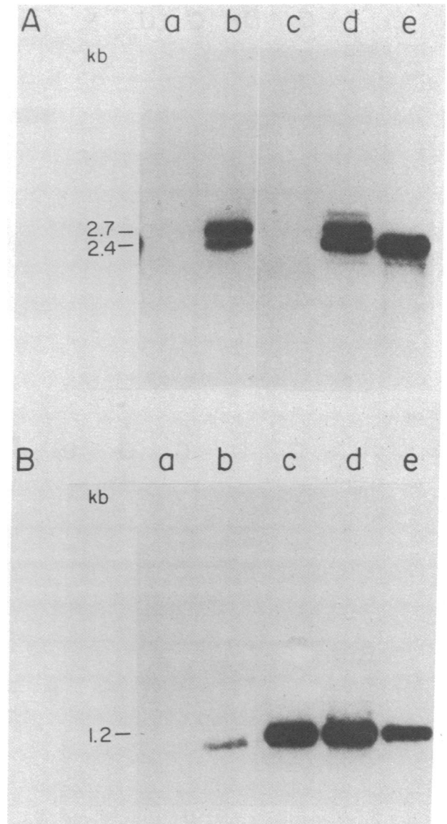
FIG. 4. Detection of \mu_{TNP} and \kappa_{TNP} gene sequences in cytoplasmic RNA from transformed cell lines. Lanes a, X63Ag8; lanes b, XR19L4; lanes c, igm-10; lanes d, IR44L1; and lanes e, Sp603. Ten micrograms of total cytoplasmic RNA (9) was denatured with glyoxal, electrophoresed through a horizontal 1% agarose gel in 10 mM sodium phosphate buffer at pH 6.9, and transferred to nitrocellulose as described by Thomas (10). (A) The blot was hybridized with a 32 P-labeled probe corresponding to the C \mu 4 exon. This probe was isolated from the cDNA clone pH76 \mu 17 (donated by J. Adams) after digestion with Pst I (18). (B) A similar blot was hybridized with a 32 P-labeled probe containing \kappa_{TNP} V-region coding sequences (16). Sizes were estimated by comparison to mouse ribosomal 28S and 18S RNA (4.7 and 2.0 kb, respectively).
