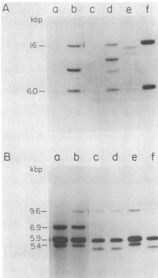
FIG. 5. Detection of pR-Sp6 and pR-HL TNP sequences in DNA from transformed cell lines. Lanes a, X63Ag8; lanes b, XR19L4; lanes c, igm-10; lanes d, IR44L1, lanes e, Sp603; and lanes f, igm-10 with 5 equivalents of pR-Sp6. Bam HI-digested DNA samples (20 μg) were electrophoresed through a 1% agarose gel at 2 V·cm -1 for 40 hr and transferred to nitrocellulose. (A) A previously hybridized blot (see B) was washed according to Thomas (10) and rehybridized to a 32 P-labeled probe containing the C μ 1 and C μ 2 exons. This probe was prepared by isolation of an appropriate fragment from a Xba I/ Hind III digestion of a genomic clone of the μ-chain constant region gene segment. The bands corresponding to the μ-chain gene-containing fragments generated by Bam HI digestion of pR-Sp6 and pR-HL TNP are indicated. The two bands observed in lane e (11 and 14 kbp) correspond to the functionally rearranged μ TNP gene in the wild-type Sp603 cell line. (B) The same blot was hybridized with a 32 P-labeled probe containing the κ-constant region gene segment that was isolated from the plasmid pL21-5 (donated by R. Wall) (22). The bands at 9.6 kb correspond to the κ TNP gene (16). The bands at 6.9, 5.9, and 5.4 kbp correspond to rearranged κ chain genes present in the DNA of the X63Ag8 cell line (23, 24), two of which (5.9 and 5.4 kbp) were retained in the generation of the original Sp6 hybridoma. The 5.4-kbp band corresponds to the functionally rearranged X63Ag8 κ gene and this band is not observed in the case of igm-10 (lane c). Sizes were estimated by comparison to Hind III-digested λ phage DNA.
