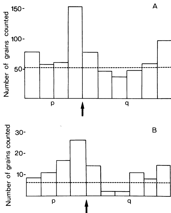
FIG. 4. Distribution of grains along chromosome 2 after in situ hybridization of [ ^3\text{H} ]cRNA transcribed from V_{\kappa} probes. p and q, short and long arms; vertical arrow, position of centromere; broken line, number of grains expected from a proportional distribution of the total number of grains on all chromosomes. (A) Distribution after hybridization to HK101 (data from Fig. 1A). (B) Distribution after hybridization to HK122 (data from 18 karyotypes).
