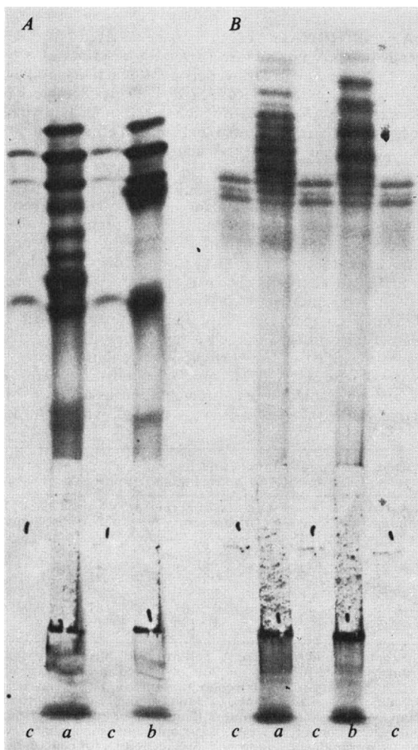
Fig. 3 Autoradiograph of labelled components secreted by anti-SRBC specific hybrid lines. Fractionation before ( B ) and after ( A ) reduction was by IEF. pH gradient was 5.0 (bottom) to 9.0 (top).
