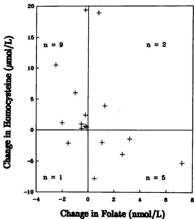
FIGURE 2 The change in plasma total homocysteine concentrations in placebo-treated subjects as function of the change in plasma folic acid concentrations. The individual changes in plasma folate concentrations were associated with opposite changes in total homocysteine concentrations ( P < 0.02 , Fisher's exact test).
