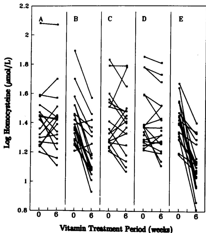
FIGURE 1 The effect of different vitamin supplements on plasma total homocysteine concentrations. Hyperhomocysteinemic men were supplemented daily for 6 wk with (A) placebo, (B) 0.65 mg folic acid, (C) 10 mg pyridoxine, (D) 0.4 mg cyanocobalamin or (E) a combination of the three vitamins. Significant declines in plasma homocysteine concentrations were observed in men supplemented with folic acid ( P < 0.001 ), cyanocobalamin ( P < 0.01 ) and the vitamin combination ( P < 0.001 ).
