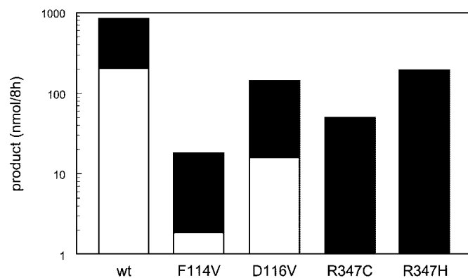
FIG. 4. Separate productions of 17-hydroxypregnenolone (■) and DHEA (□) from 1 \mu M pregnenolone by the COS-1 cells described in Fig. 2A. Note the logarithmic y-axis.
