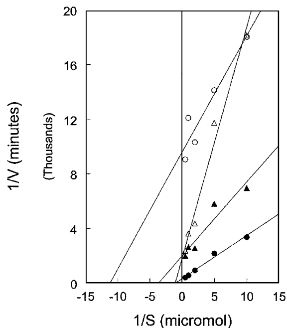
FIG. 3. Lineweaver-Burk plot for the conversion of pregnenolone to 17-hydroxypregnenolone plus DHEA, shown in Fig. 2A, by wild-type CYP17 (●), and the D116V (△), R347C (○), and R347H (▲) mutants. Results for the F114V mutant are not shown, because all measured values are outside the axes used.
