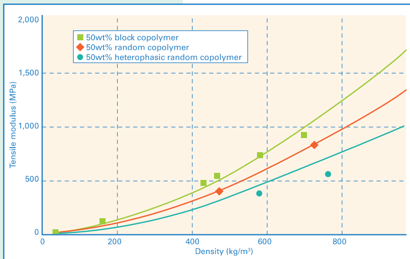
Figure 9: Experimental data for the tensile modulus of various Daploy HMS-PP blends and theoretical curves
