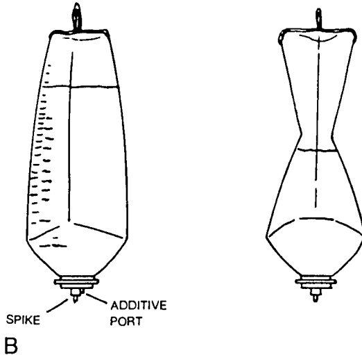
Figure 8-16. A, Abbott (LifeCare) and Travenol (Viaflex) supply nonvented polyvinyl-chloride flexible plastic containers. These containers require nonvented sets. B, McGaw (Accumed) offers a nonvented semi-rigid polyolefin plastic container.
