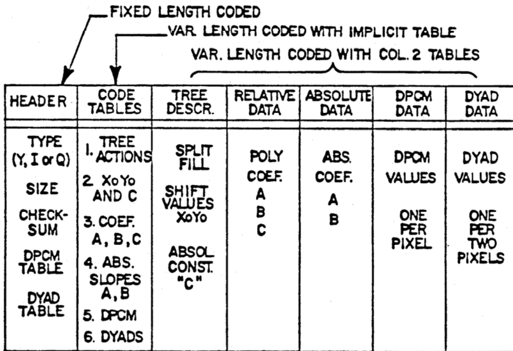
STREAM FORMAT FOR EACH OF Y, I AND Q SUBFRAMES
