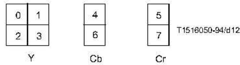
Figure 6-11 – 4:2:2 Macroblock structure
