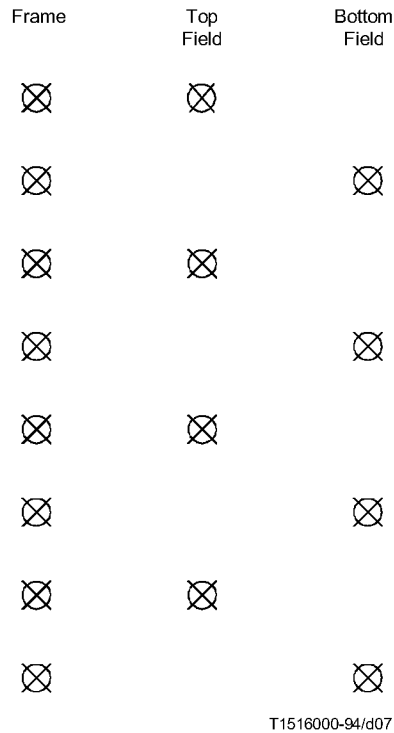
Figure 6-6 – Vertical positions of samples with 4:2:2 and 4:4:4 data
