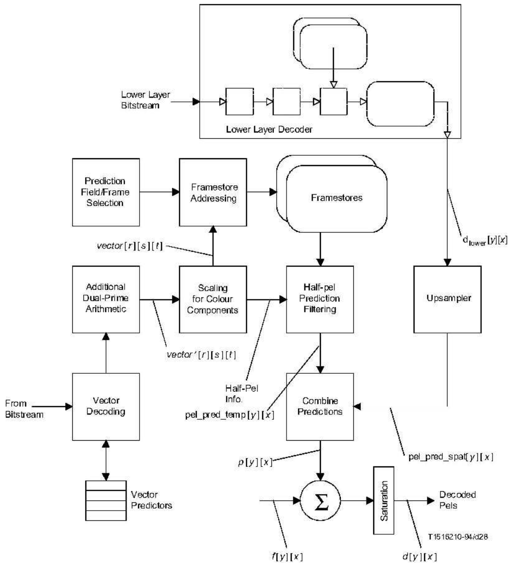
Figure 7-13 – Simplified motion compensation process for spatial scalability
