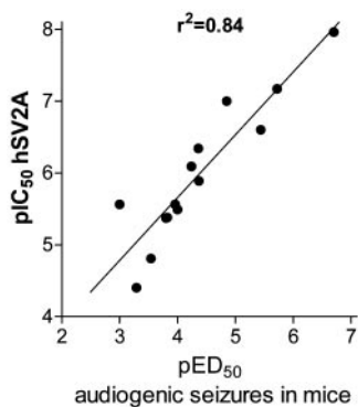
Fig. 6. Correlation between binding affinity and antiseizure potency of LEV derivatives. Correlation of binding of a series of LEV-related compounds to hSV2A assayed in transiently transfected COS-7 cells (pIC 50 s measured by using [ 3 H]ucb 30889), and of antiseizure potencies shown as the -\log ED 50 s (pED 50 s) in the mouse audiogenic seizure model. There is a good correlation between antiseizure potency in audiogenic mice and affinity to hSV2A.
