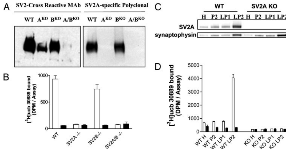
Fig. 2. Binding of [ 3 H]ucb 30889 to WT and KO brain membranes and synaptic vesicles. (A) Western blot of brain membranes from WT and homozygous KO mice probed with an anti-SV2 monoclonal antibody (cross-reactive to all isoforms) or with an anti-SV2A-specific polyclonal antibody. Lanes 1, WT; lanes 2, SV2A -/- KO; lanes 3, SV2B -/- KO; lanes 4, SV2A -/- /B -/- double KO. (B) Binding of [ 3 H]ucb 30889 to brain membranes from WT, SV2A -/- , SV2B -/- , and SV2A -/- /SV2B -/- KO mice. Binding is observed only to membranes from animals expressing SV2A. □, [ 3 H]ucb 30889 alone; ■, [ 3 H]ucb 30889 plus 1 mM LEV. Error bars are the SD of experiments performed with five WT brains and four KO brains, with three replicates within each experiment. (C) Purification of synaptic vesicles enriches for the synaptic vesicle proteins and LEV binding. Shown are blots of mouse brain homogenate (H), crude synaptosomes (P2), plasma and heavy membranes (LP1), and synaptic vesicles (LP2) (2 μg of each fraction) that were probed for the synaptic vesicle proteins SV2A (Upper) and synaptophysin (Lower). The synaptic vesicle fraction from WT animals displays enrichment of both synaptic vesicle proteins and LEV-binding proteins, whereas material from SV2A KOs shows enrichment of synaptophysin only. (D) Binding to the different fractions using [ 3 H]ucb 30889 shows significant binding only to the WT LP2 fraction, containing SV2A-rich synaptic vesicles. Shown are [ 3 H]ucb 30889 alone (open bars) and [ 3 H]ucb 30889 plus 1 mM LEV (filled bars). Shown are representative examples of two experiments. Error bars are the SD of two replicates.
