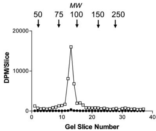
Fig. 1. Photolabeling of the LEV-binding site in synaptic vesicles from rat brain. After photoaffinity labeling with [ 3 H]ucb 30889, SDS-solubilized proteins were run on an SDS/PAGE gel, and then the gel was cut into thin slices and counted for 3 H content. Photoaffinity labeling of crude synaptosomal (P2) (●) and synaptic vesicle (LP2) (□) fractions by using [ 3 H]ucb 30889 is shown. Photoaffinity labeling identifies a protein of ≈90 kDa enriched in the synaptic vesicle fraction.
