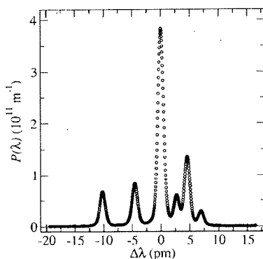
FIG. 4. Line profile function of the 2p_0 \leftrightarrow 1s_3 transition in Xe obtained at
