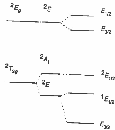
Figure 11.6 The energy band diagram for Ti:sapphire.
