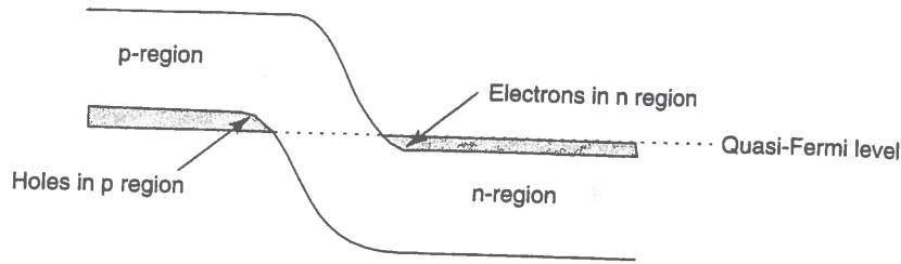
Figure 12.32 In equilibrium, the quasi-Fermi levels of the degenerate p- and n-junction laser material align.
