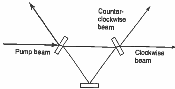
Figure 11.10 One of the advantages of a ring laser is that it is relatively easy to configure the resonator so that the back-reflected beam from a pump laser is not reflected into the resonator of the pump laser.
