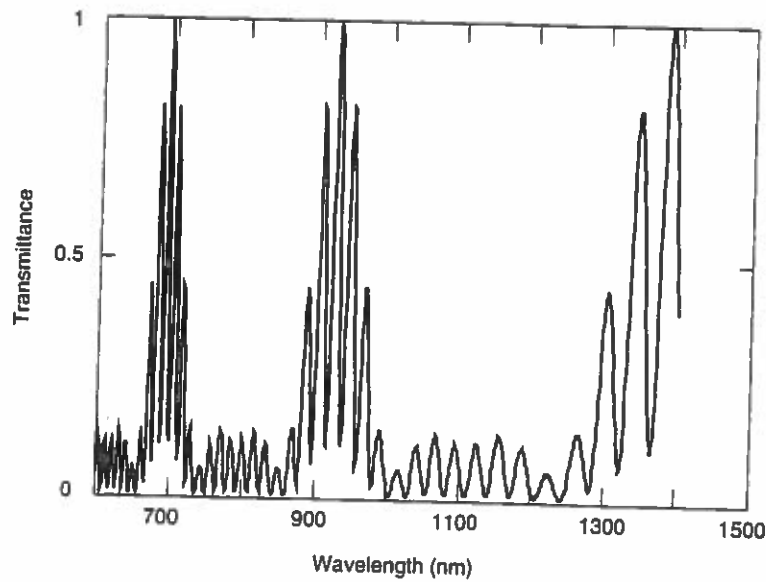
Figure 11.20 Multiple birefringent filters can be used to provide greater selectivity. This illustrates the transmittance of a three-stage birefringent filter with thicknesses of 0.5 mm, 1 mm, and 7.5 mm.
