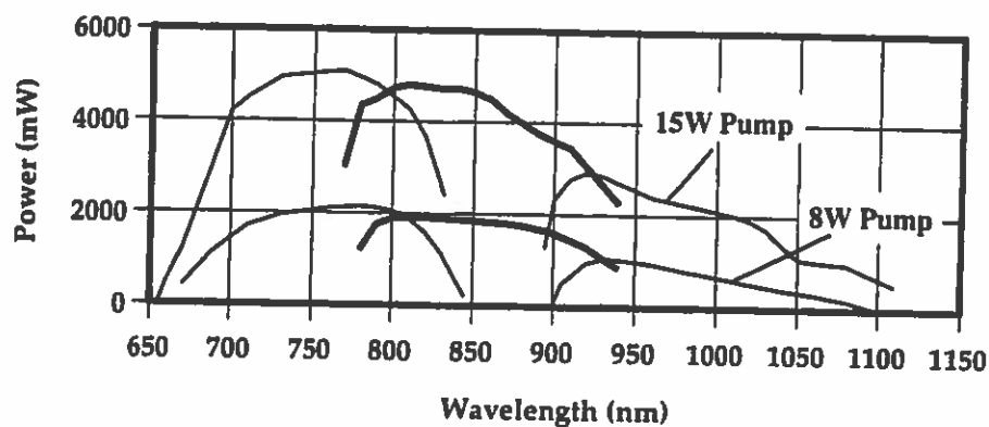
Figure 11.22 The Coherent Model 890 laser is a laser-pumped cw broadband Ti:sapphire laser. Three sets of standard optics are used to access the Ti:sapphire tuning range. Using these three sets of optics, the wavelength can be tuned from 690 nm to beyond 1100 nm. (Courtesy of the Coherent, Inc., Laser Group, Santa Clara, CA)
