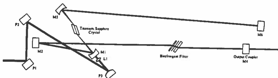
Figure 11.23 The Model 890 resonator is a folded linear resonator. (Courtesy of the Coherent, Inc., Laser Group, Santa Clara, CA)
