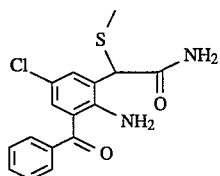
Compound 4 2-Amino-3-benzoyl-5-chloro- \alpha -(methylthio)-phenylacetamide
