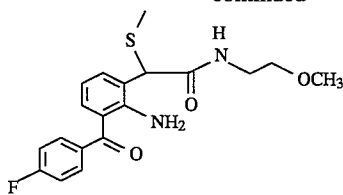
Compound 5 2-Amino-3-(4-fluorobenzoyl)- \alpha -(methylthio)-N-(2-methoxyethyl)acetamide
