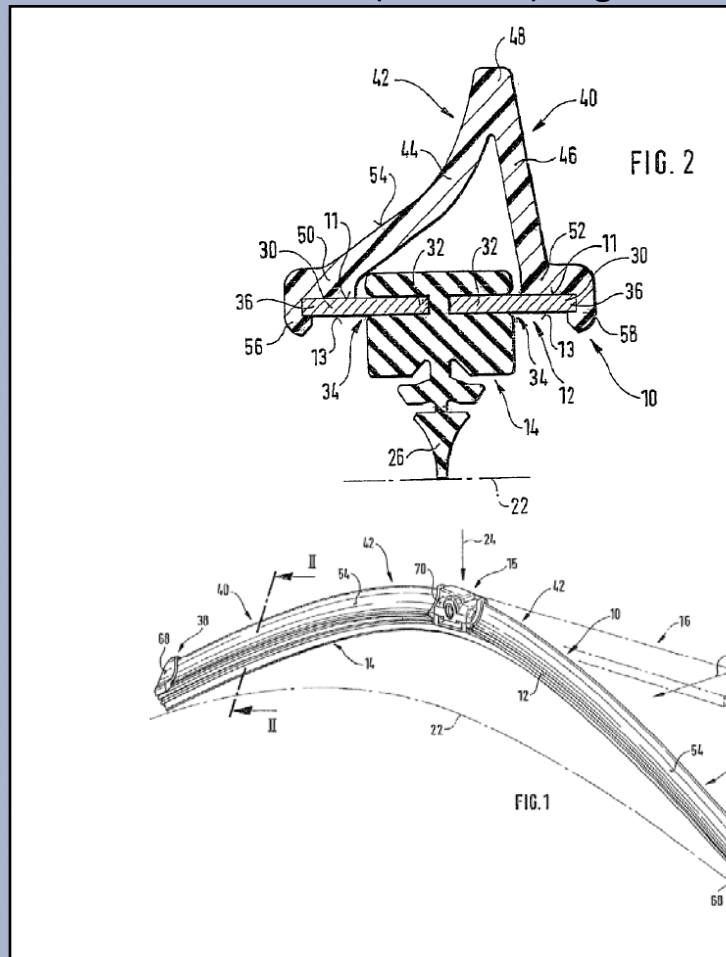
'905 Patent (Ex. 1001), Figs. 1 & 2
