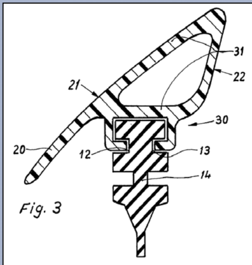
Prohaska (Ex. 1003), Fig. 3
