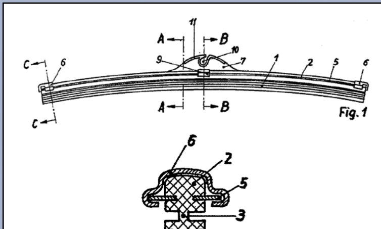
Hoyler (Ex. 1004), Fig. 1 & cross-section C-C
