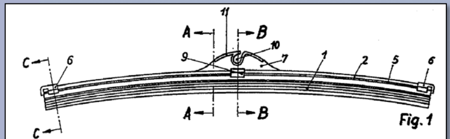
Hoyler (Ex. 1004), Fig. 1 & cross-section
