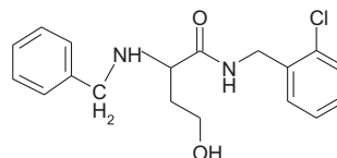
N-( o -chlorobenzyl)-amide of \alpha -(benzylamine)- \gamma -hydroxybutyric acid ( IX )
