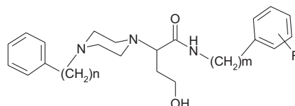
\alpha -(4-Phenylpiperazine)- \gamma -hydroxybutyric acid and \alpha -(4-benzylpiperazine)- \gamma -hydroxybutyric acid derivatives ( X )
