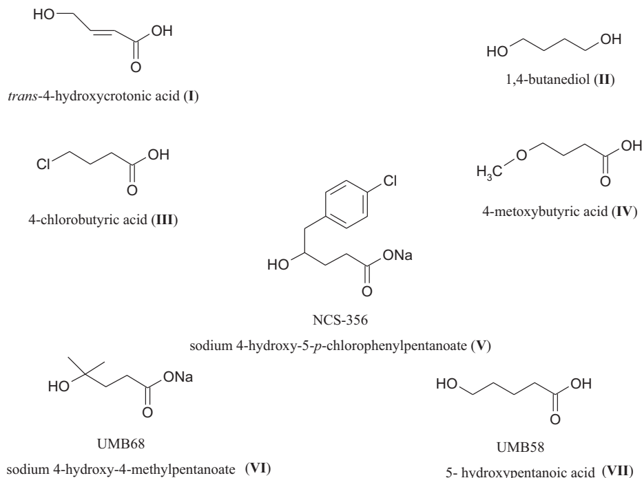
Fig. 3. GHB-related compounds
