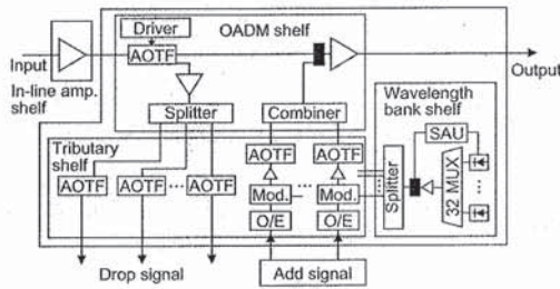
Figure 5 OADM configuration using AOTFs.
