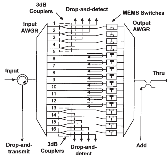
Fig. 1. Reconfigurable drop module with channels 1–4 and 13–16 arranged for DD and channels 5–12 arranged for DT. Arbitrary reconfiguration of all 16 channels is obtained using voltage-actuated silicon MEM's optical switches.
