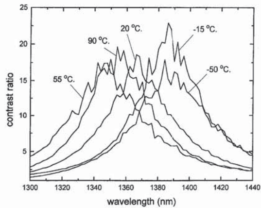
Fig. 8. Modulator contrast ratio spectra at temperatures from -50^\circ\text{C} to 90^\circ\text{C} .
