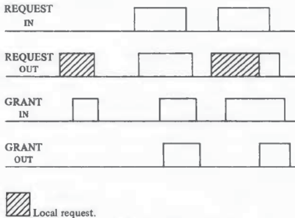
FIGURE 3.10 Daisy-chain timing.
