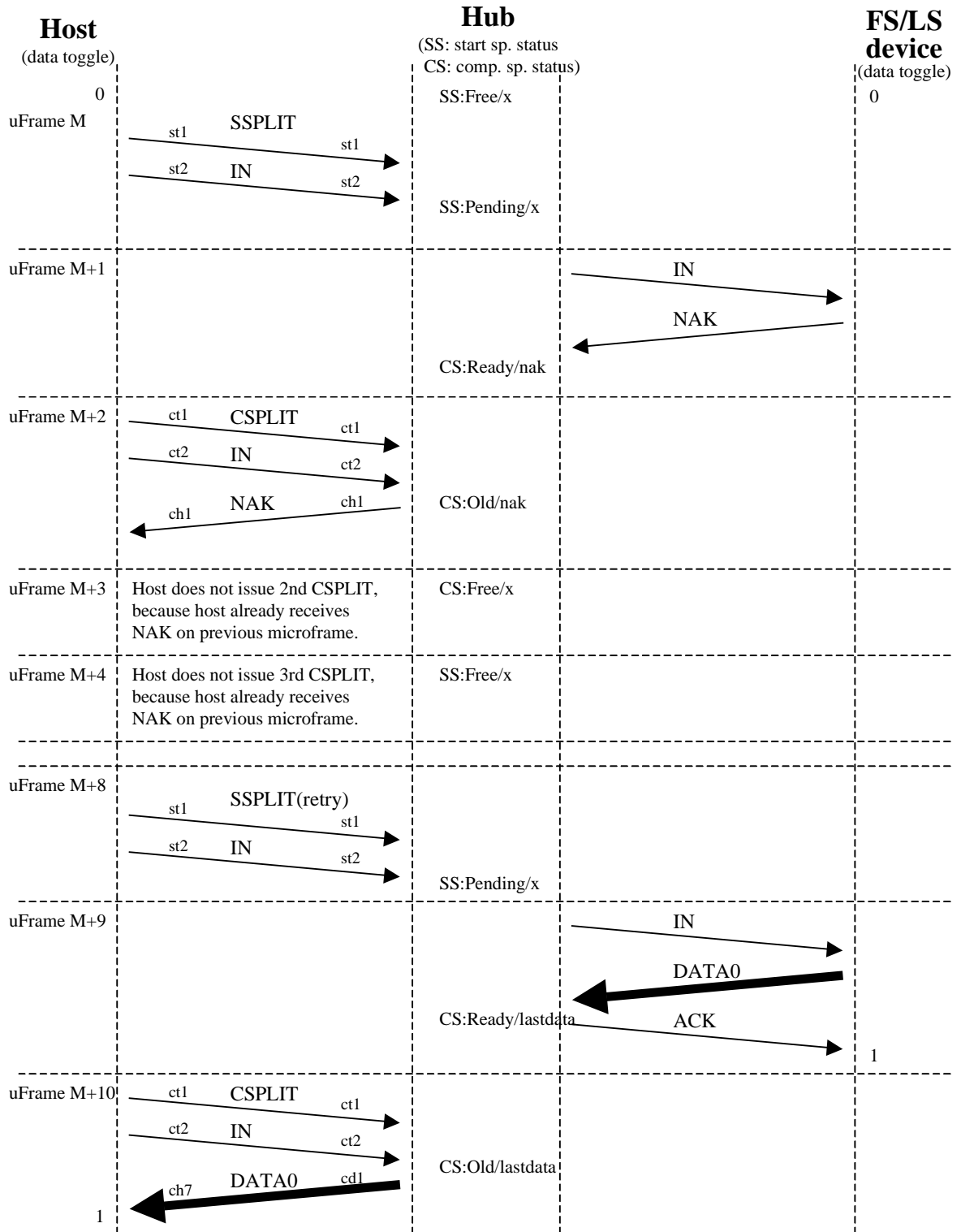
Figure A-82. Device Busy No Smash (FS/LS NAK)
