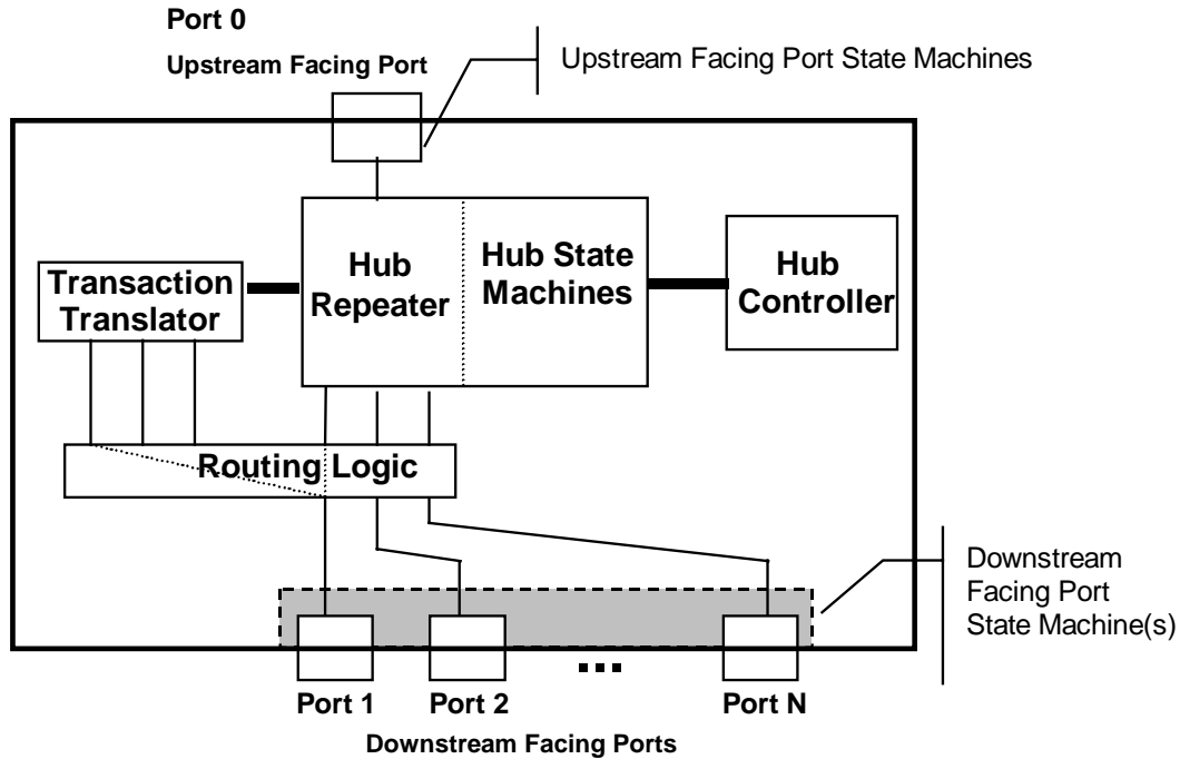
Figure 11-1. Hub Architecture
