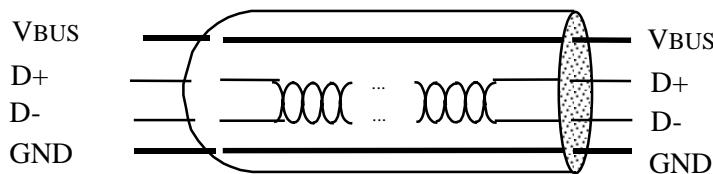
Figure 4-2. USB Cable
