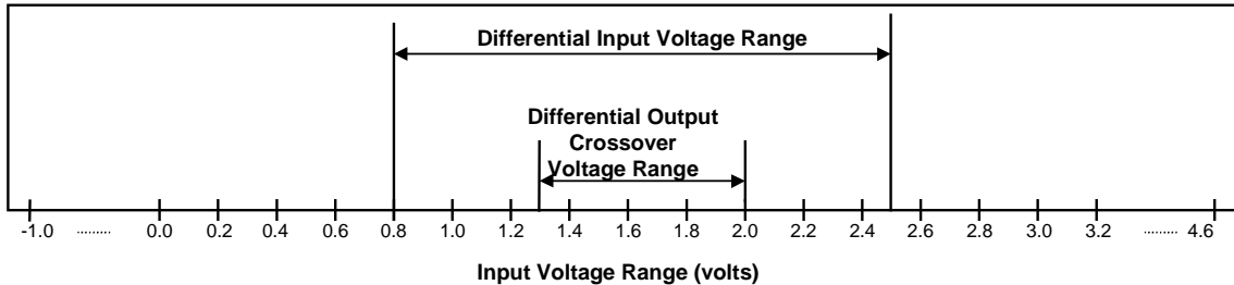
Figure 7-19. Differential Input Sensitivity Range for Low-/full-speed
