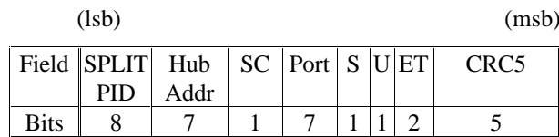
Figure 8-12. Complete-split (CSPLIT) Transaction Token
