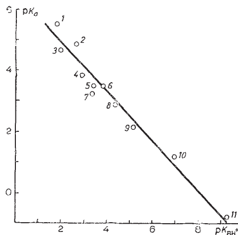
Fig. 1. Dependence of the pK_a and pH_{BH}^* values of 5-substituted tetrazoles: 1) 5-methyltetrazole; 2) tetrazole; 3) 5-(p-methoxyphenyl)tetrazole; 4) 5-(m-chlorophenyl)tetrazole; 5) (m-nitrophenyl)tetrazole; 6) 5-(p-nitrophenyl)-tetrazole; 7) 5-(o-nitrophenyl)tetrazole; 8) 5-iodotetrazole; 9) 5-bromotetrazole; 10) 5-trifluoromethyltetrazole; 11) 5-nitrotetrazole.
