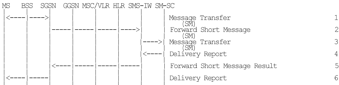
Figure 53: MO SMS Transfer, Successful
