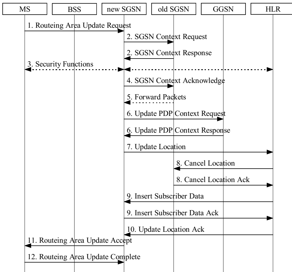
Figure 27: Inter SGSN Routeing Area Update Procedure
