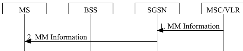
Figure 16: MM information Procedure
