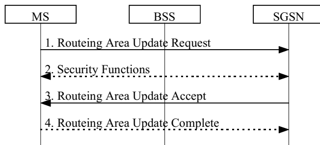
Figure 26: Intra SGSN Routeing Area Update Procedure
