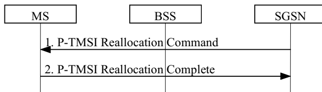
Figure 23: P-TMSI Reallocation Procedure
