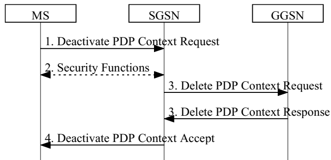
Figure 40: PDP Context Deactivation Initiated by MS Procedure
