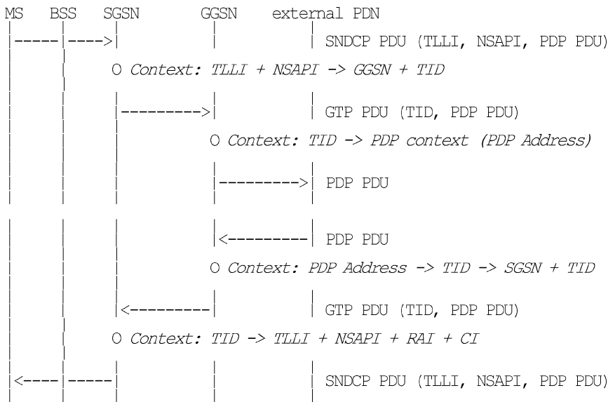
Figure B.1: Data Routing in HPLMN to and from an External PDN
