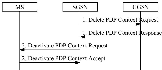
Figure 41: PDP Context Deactivation Initiated by SGSN Procedure
