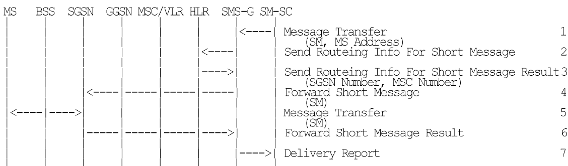
Figure 51: MT SMS Transfer, Successful
