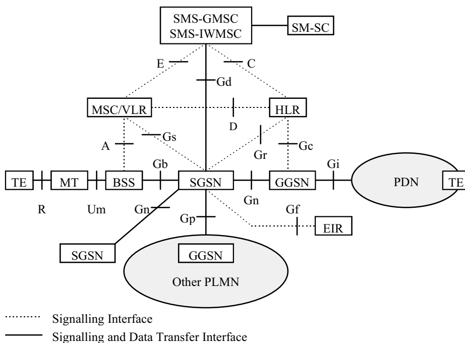
Figure 2: Overview of the GPRS Logical Architecture
