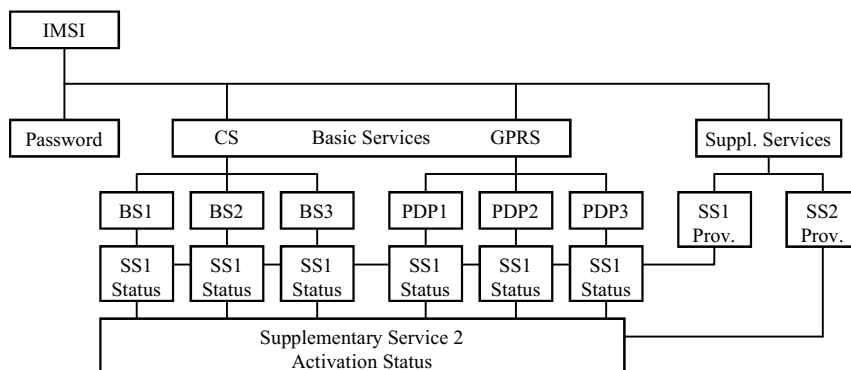
Figure 49: GPRS Subscription Data
