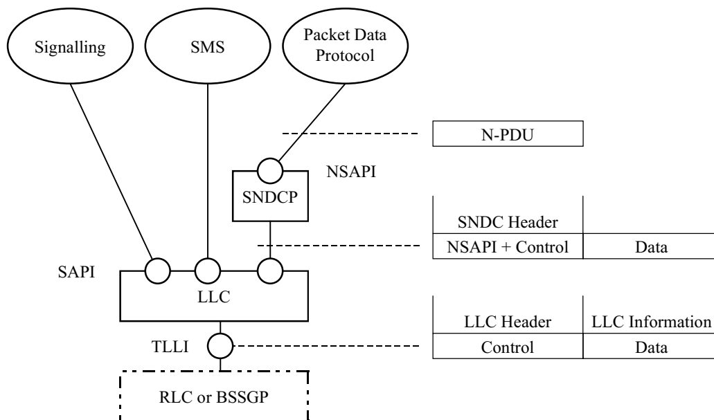
Figure 45: Multiplexing of Network Protocols
