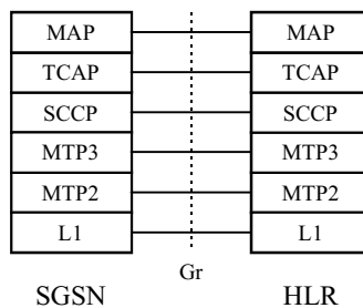
Figure 6: Signalling Plane SGSN - HLR
