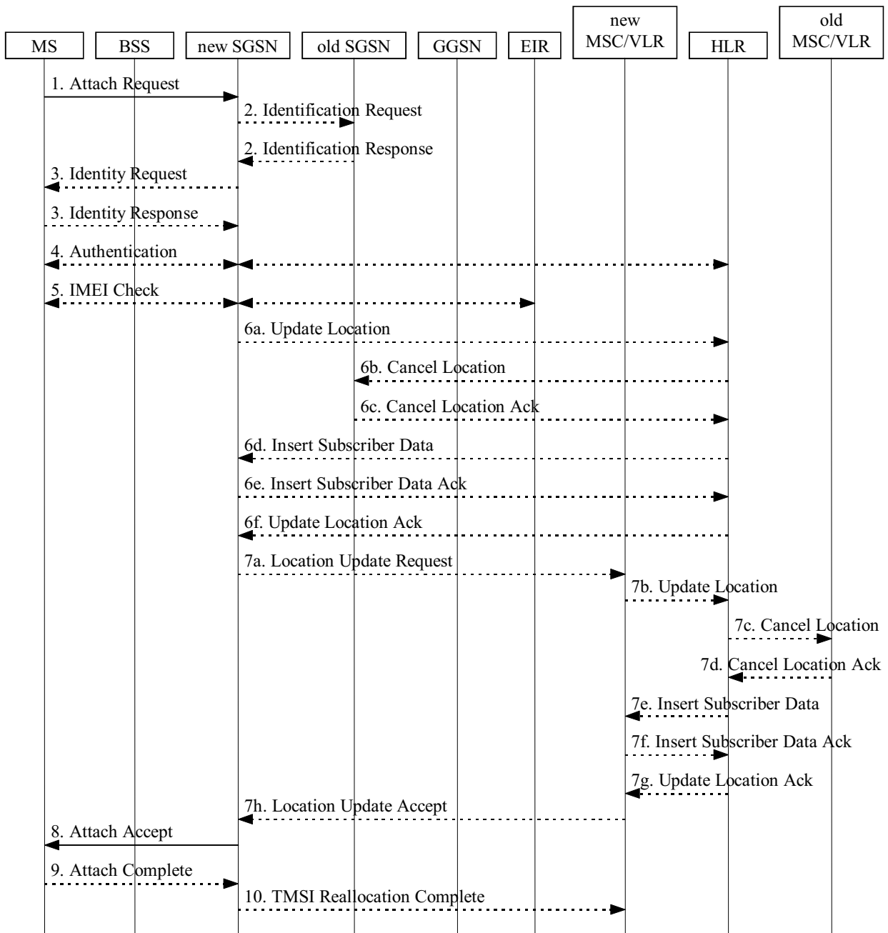
Figure 17: Combined GPRS / IMSI Attach Procedure
