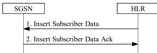
Figure 30: Insert Subscriber Data Procedure
