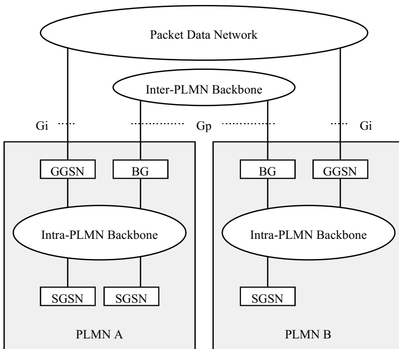
Figure 3: Intra- and Inter-PLMN Backbone Networks
