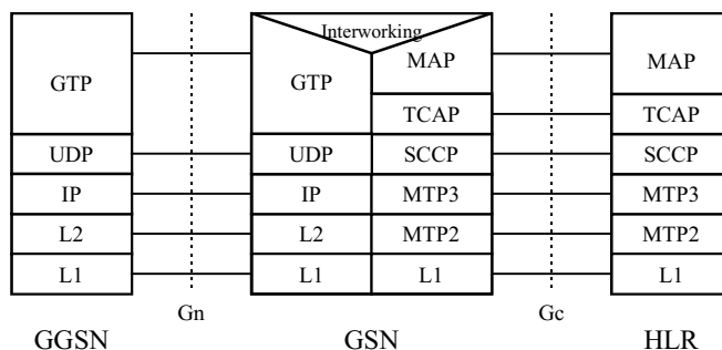
Figure 11: Signalling Plane GGSN - HLR Using GTP and MAP
