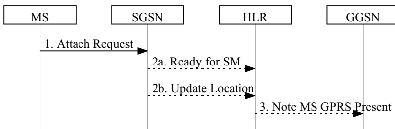
Figure 37: Mobile User Activity Procedure
