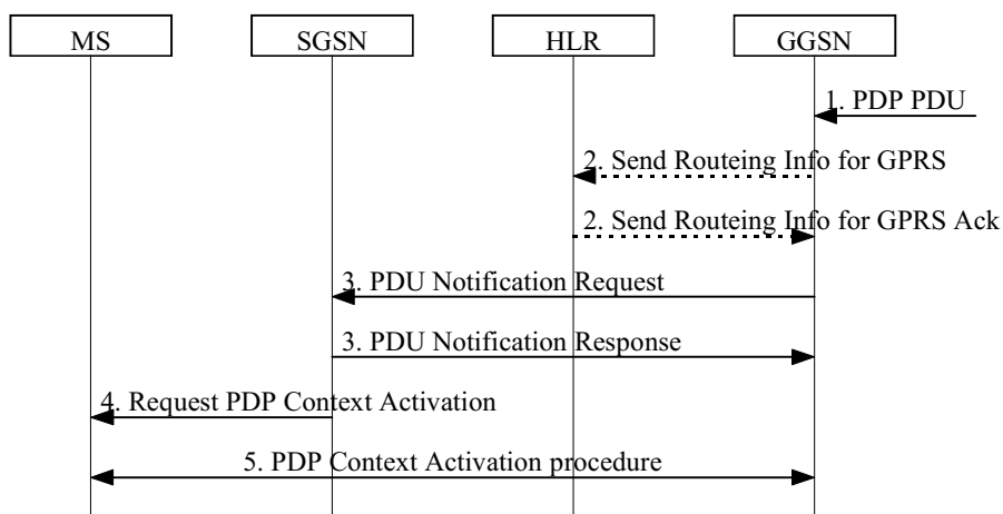
Figure 35: Successful Network-Requested PDP Context Activation Procedure
