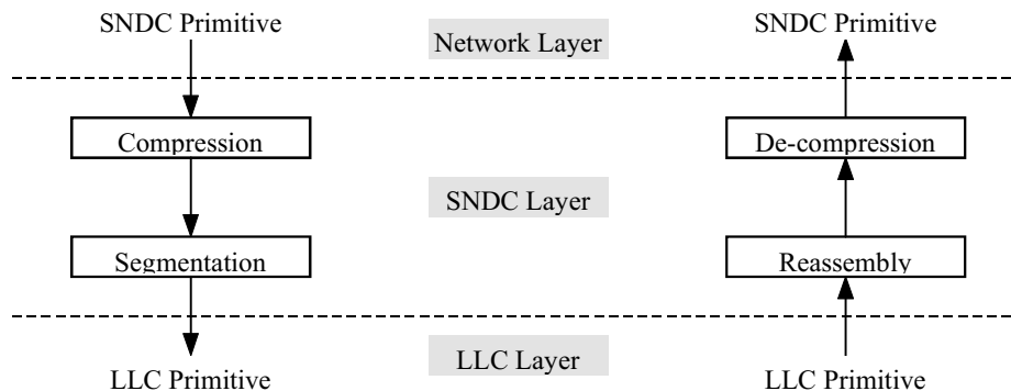
Figure 46: Sequential Invocation of SNDC Functionality
