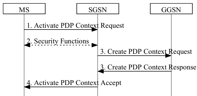
Figure 34: PDP Context Activation Procedure
