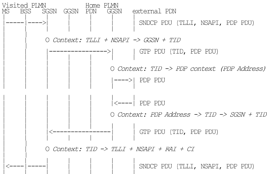
Figure B.2: Data Routing for a Roaming MS to and from an External PDN
