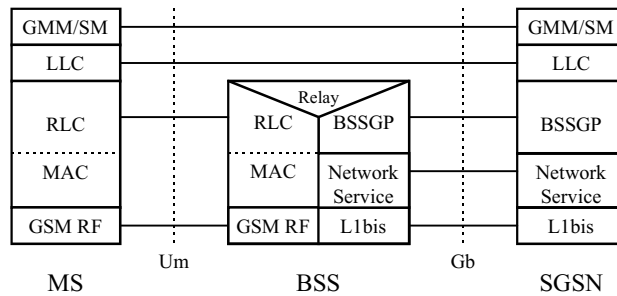
Figure 5: Signalling Plane MS - SGSN
