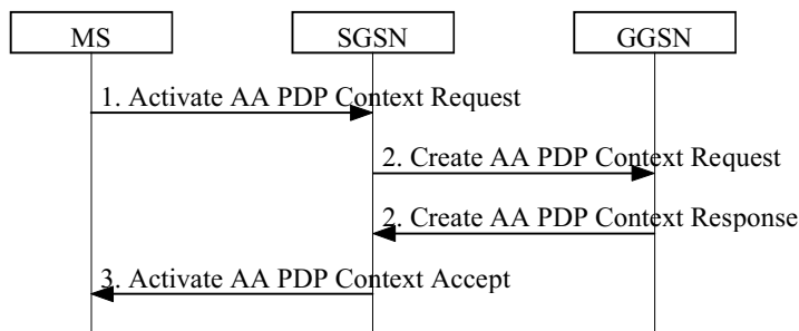
Figure 38: Anonymous Access PDP Context Activation Procedure
