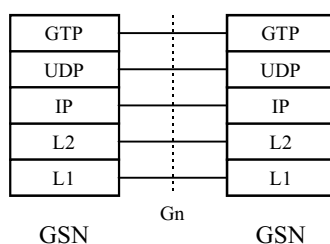
Figure 9: Signalling Plane GSN - GSN
