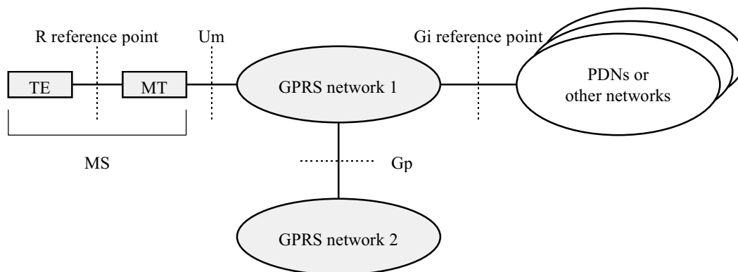
Figure 1: GPRS Access Interfaces and Reference Points
