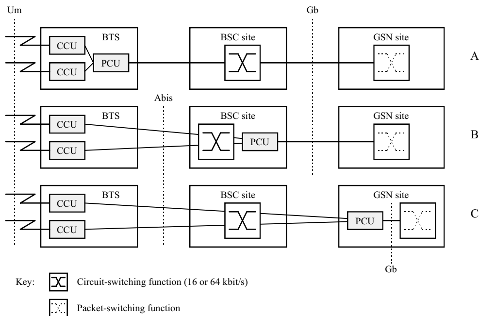
Figure 48: Remote Packet Control Unit (PCU) Positions
