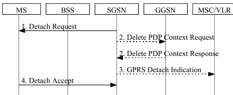
Figure 19: SGSN-Initiated GPRS Detach Procedure
