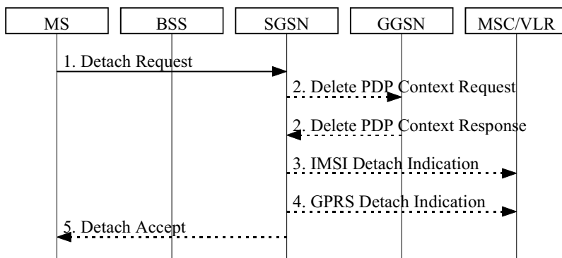
Figure 18: MS-Initiated Combined GPRS / IMSI Detach Procedure
