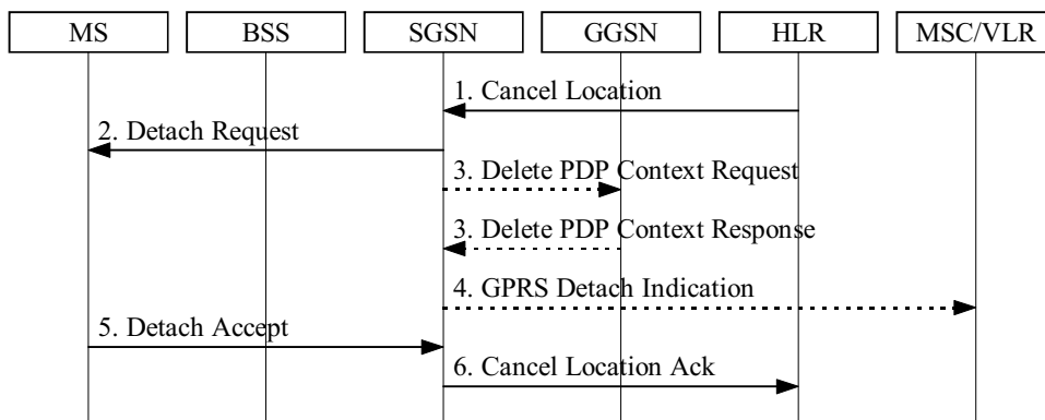
Figure 20: HLR-Initiated GPRS Detach Procedure
