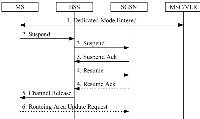
Figure 54: Suspend and Resume Procedure
