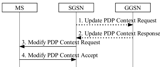
Figure 39: PDP Context Modification Procedure
