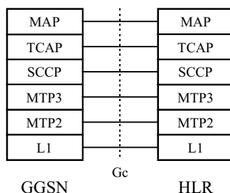
Figure 10: Signalling Plane GGSN - HLR Using MAP
