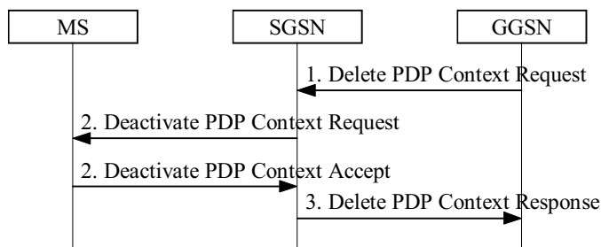
Figure 42: PDP Context Deactivation Initiated by GGSN Procedure
