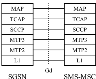
Figure 8: Signalling Plane SGSN - SMS-GMSC and SGSN - SMS-IWMSC
