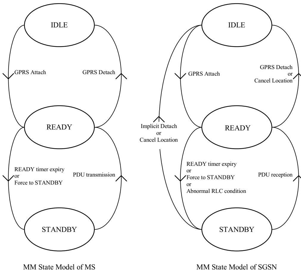
Figure 12: Functional Mobility Management State Model
