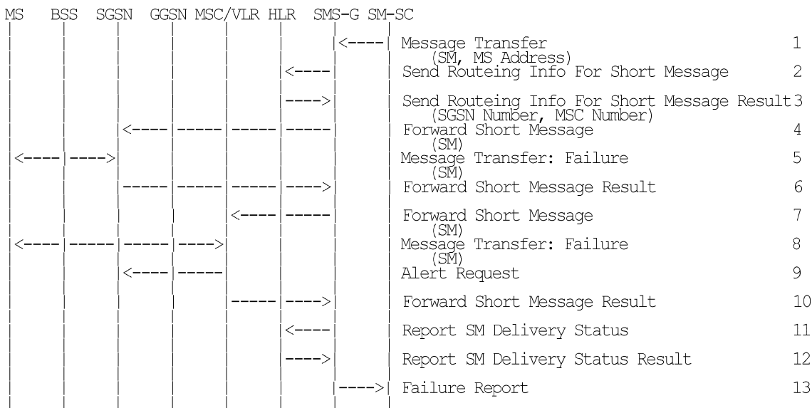
Figure 52: MT SMS Transfer, Unsuccessful
