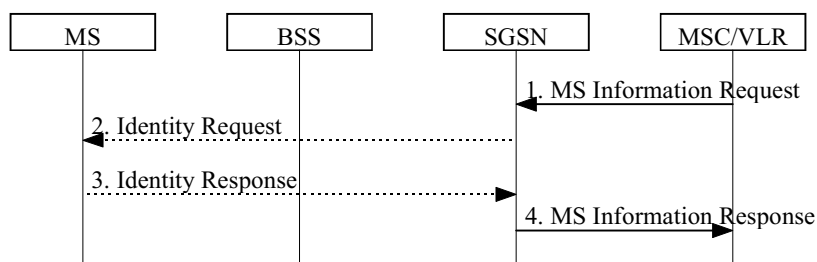
Figure 15: MS Information Procedure
