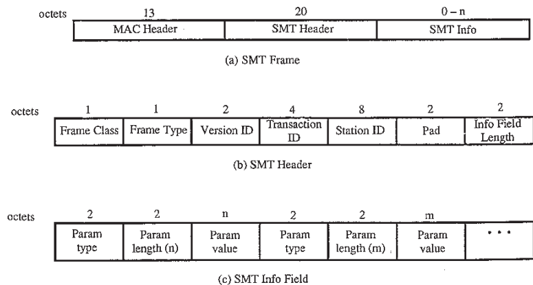
FIGURE 11.8 SMT Frame Format
