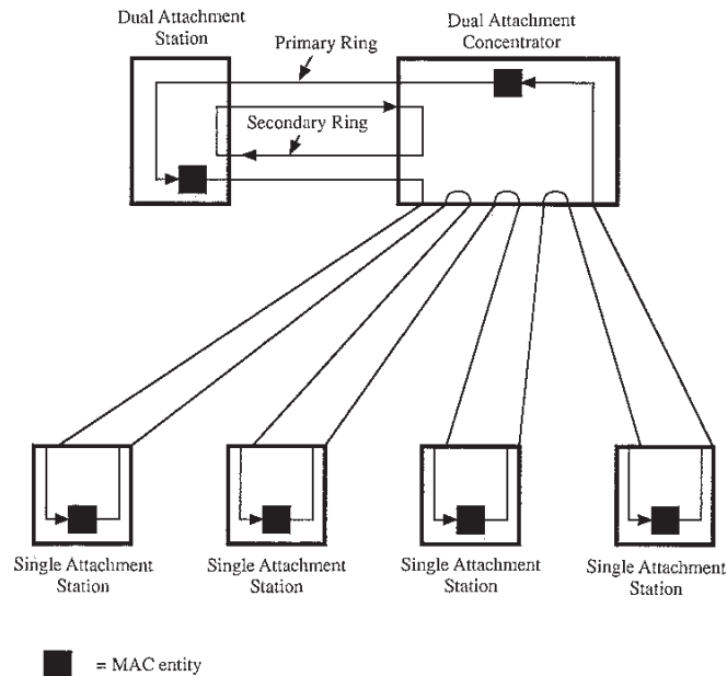
FIGURE 6.9 Star-Shaped Ring
