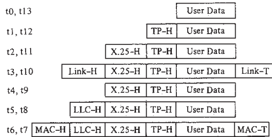
(b) Operation
