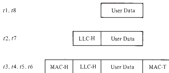
(b) Operation
