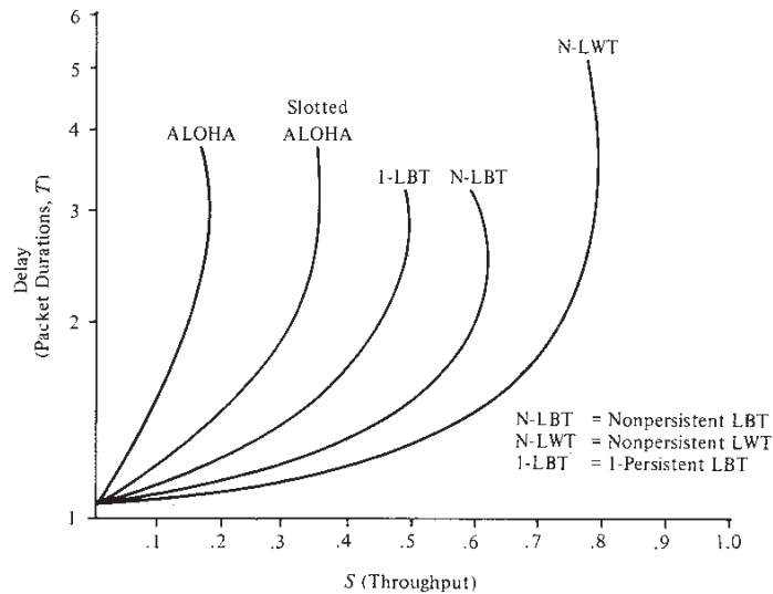
FIGURE 9.16 Delay for Various Contention Protocols
