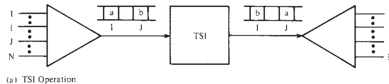
(a) TSI Operation
