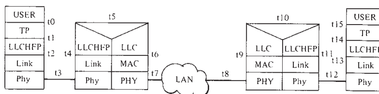
(a) Architecture
