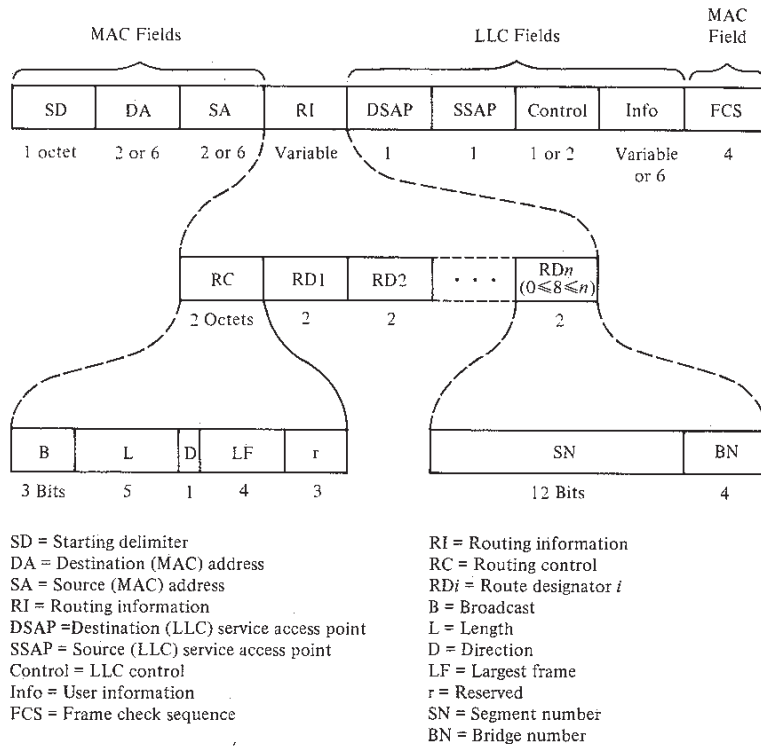
FIGURE 10.16 Source Routing Formats
