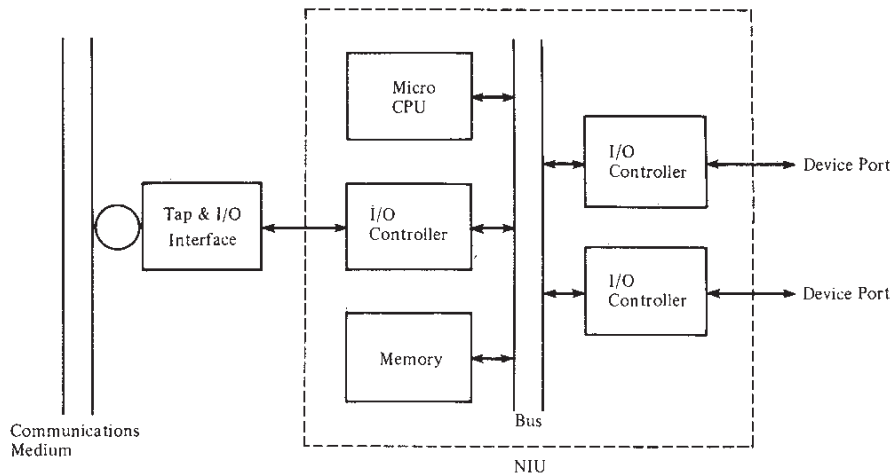
FIGURE 8.3 NIU Architecture
