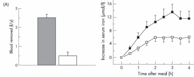
Figure 2 Influence of proton pump inhibitors (PPIs) on iron absorption. (A) Need for venesection in haemochromatosis patients before (closed bar) and during PPI therapy (open bar). (B) Reduced serum iron levels after an iron-containing meal off (closed points) and on a PPI (open points). Reproduced with permission from Hutchinson et al. 43
