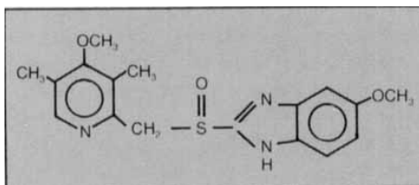
Figure 1. Omeprazole, H 168/68, 5-methoxy-2-[[[4-methoxy-3,5-dimethyl-2-pyridinyl] methyl] sulfinyl]-1H-benzimidazole.
