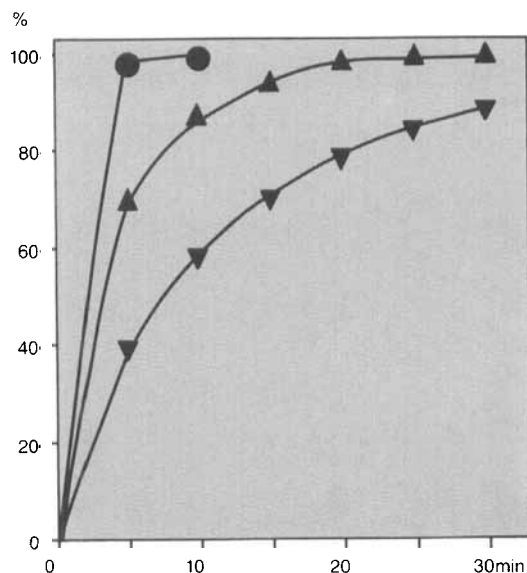
Figure 3. Dissolution of omeprazole from three granule formulations in vitro in phosphate buffer, pH= 6.5. The cumulative amount dissolved (%) is plotted as a function of time.
