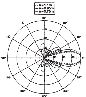
Figure 11: Antenna patterns versus array radius.
