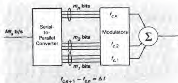
Fig. 1. Basic multicarrier transmitter.
