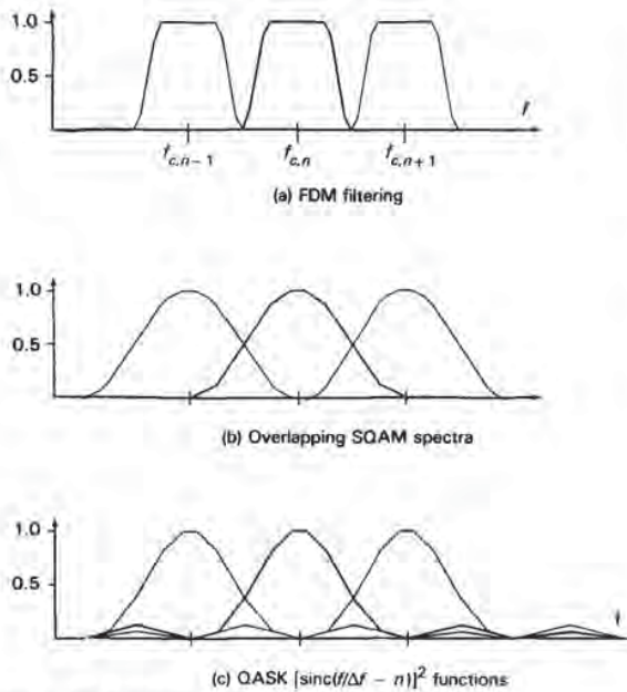
Fig. 2. MCM transmit power spectra.
