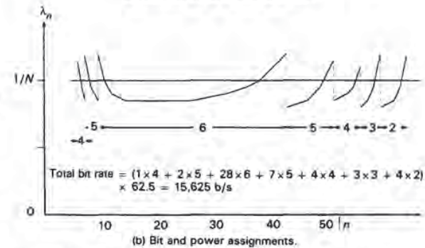
Fig. 3. Adaptive loading for a badly distorted GSTN channel.
