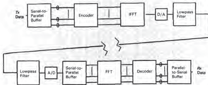
Fig. 7. Basic multicarrier "mo-dem."
