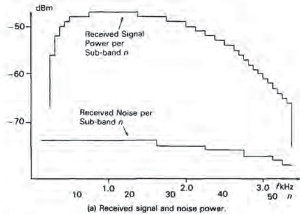
(a) Received signal and noise power.
