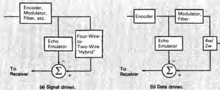
Fig. 8. Echo cancelers.
