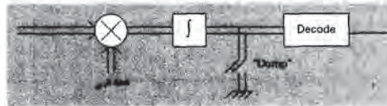
Fig. 4. Integrate and dump detection for QASK.
