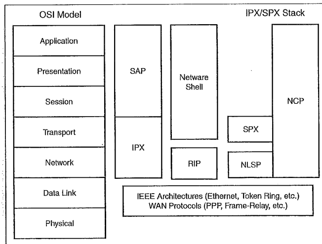
FIGURE 12.1 The IPX/SPX protocol is a routable stack made up of several protocols.
