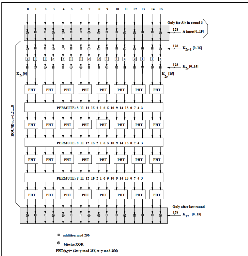
Figure 14.13: One round in A_r and A_r . The permutation boxes show how input byte indices are mapped onto output byte indices. Thus, position 0 (leftmost) is mapped on position 8, position 1 is mapped on position 11, et cetera.
