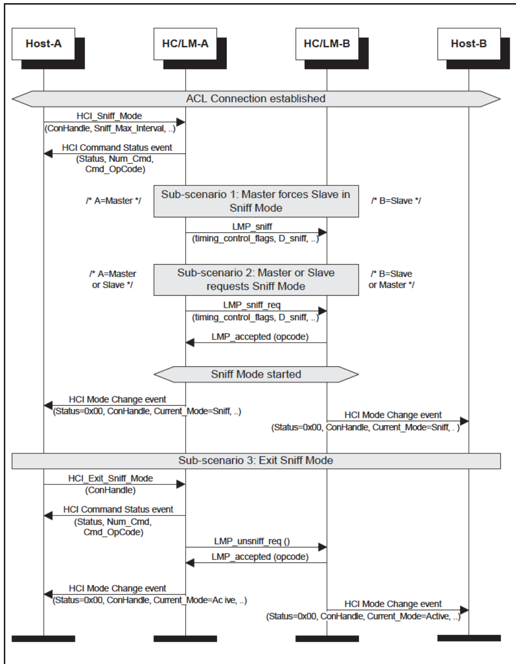
Figure 6.1: Sniff Mode
