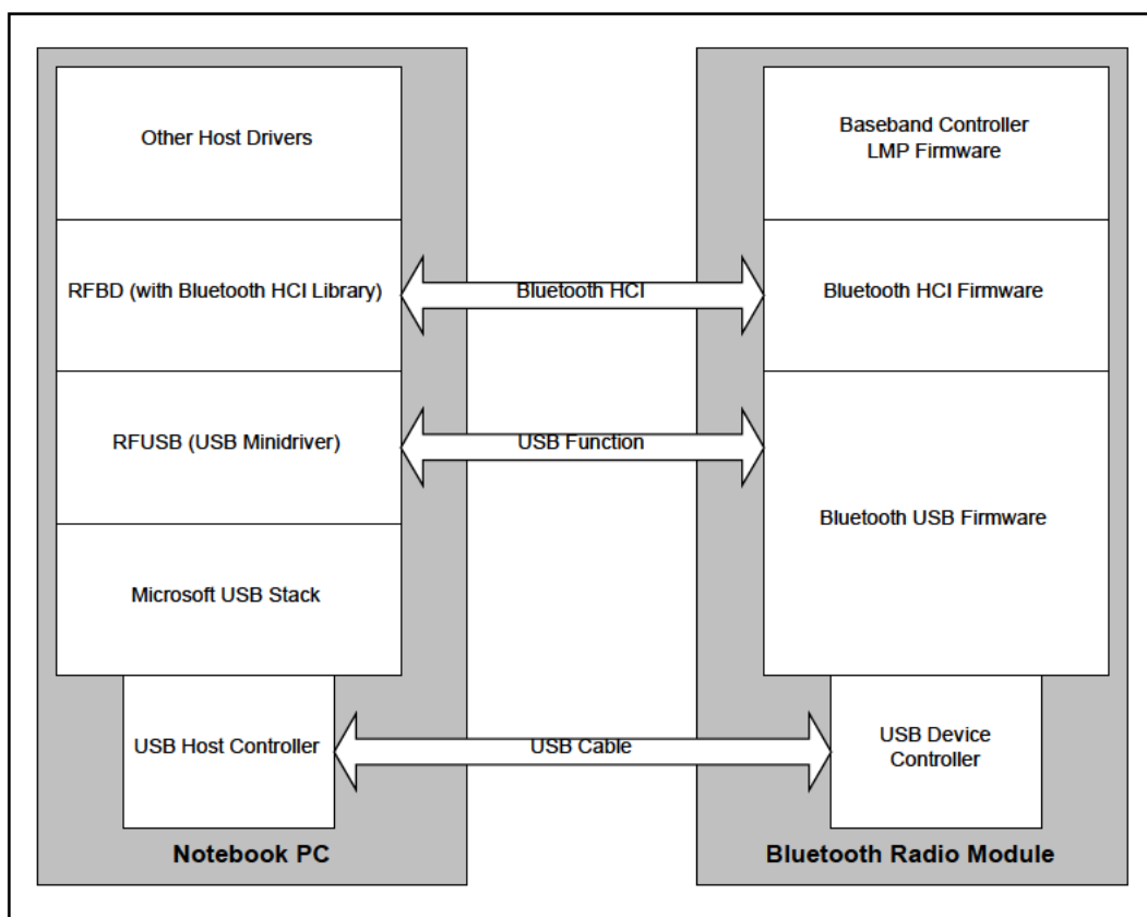
Figure 1.1: The Figure illustrates the relationship between the host and the Bluetooth Radio Module
