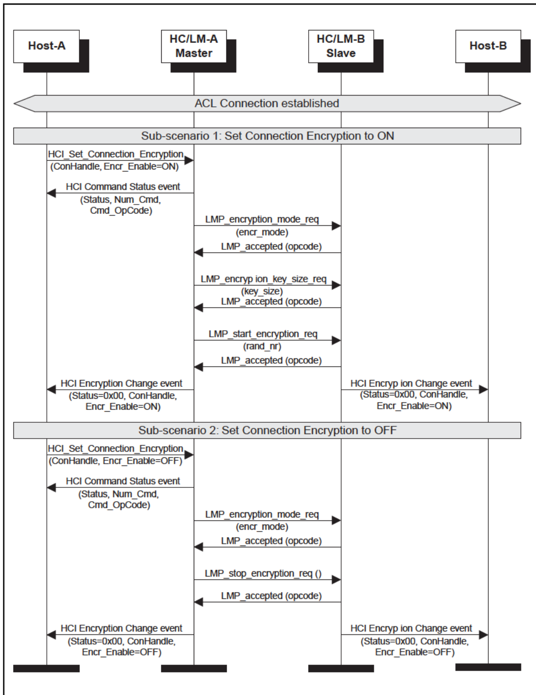
Figure 4.2: Set Connection Encryption
