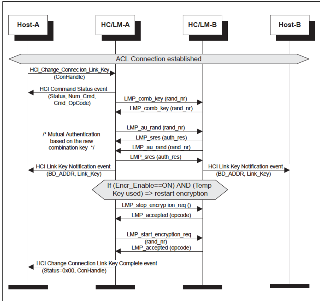
Figure 4.3: Change Connection Link Key
