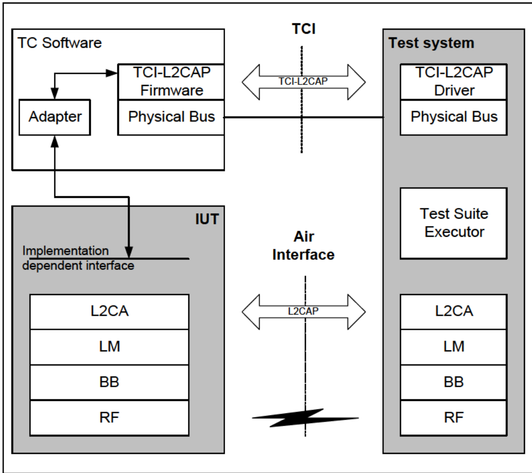
Figure 2.4: L2CAP verification
