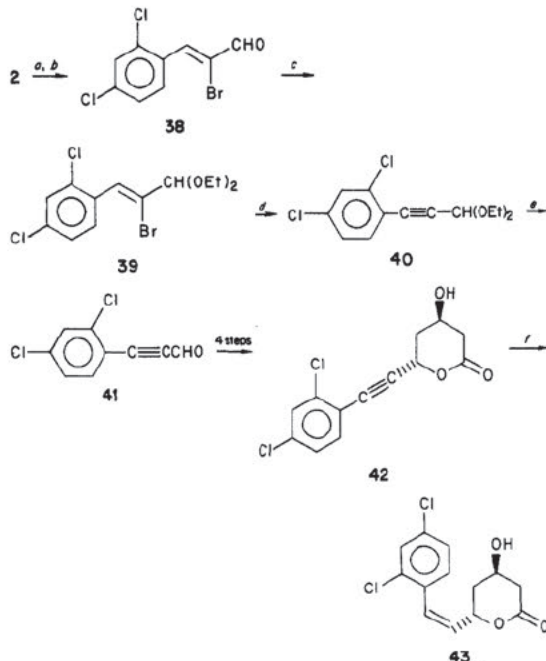
Scheme VIII
