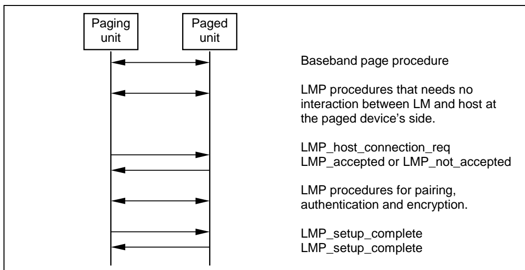
Figure 4.1: Connection establishment.
