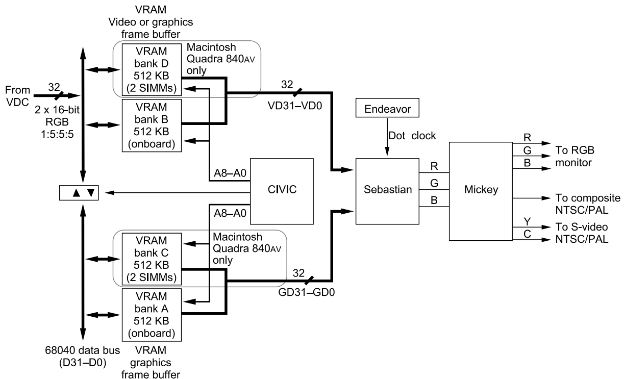
Figure 2-7 Video and graphics output system block diagram
