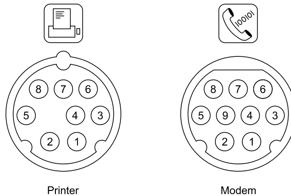
Figure 2-3 Serial port connectors
