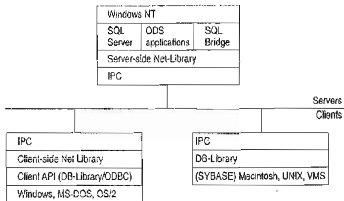
Figure 8.2 Net-Library Architecture
