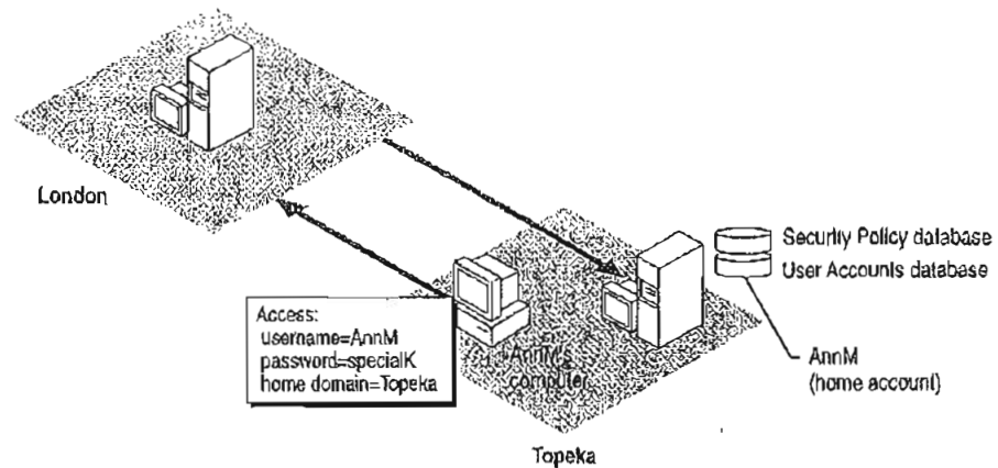
Figure 4.6 Pass-Through Authentication
