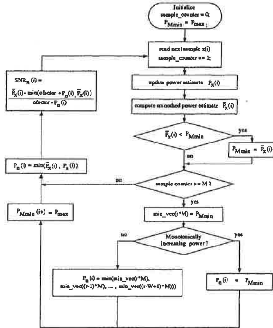
Figure 2: Flowchart of the SNR estimation algorithm
