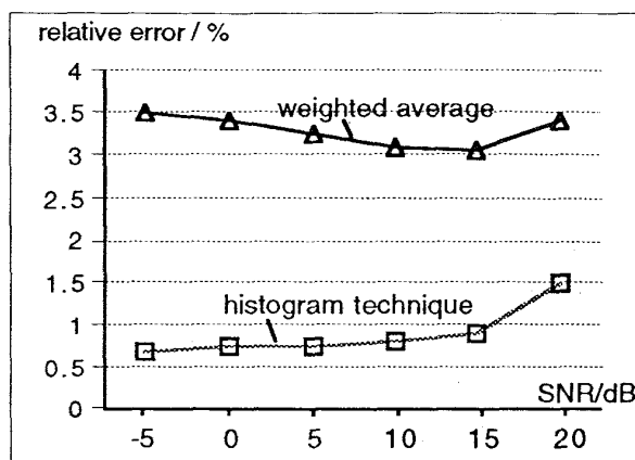
Fig. 2. Relative error for the estimation of the noise power spectrum with both techniques at different SNRs
