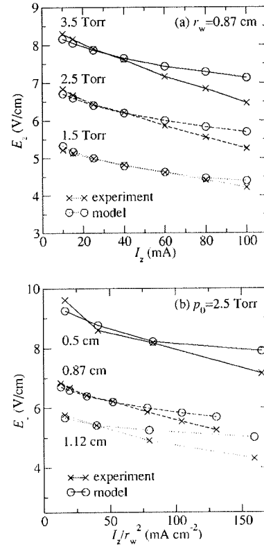
FIG. 7. Experimental data (crosses) and data predicted by the model (circles) for the axial electric field strength E_z as a function of the discharge current I_z for three different gas pressures p_0 and a tube radius r_w = 0.87 cm (a) and for three different tube radii in the case of p_0 = 2.5 Torr (b).
