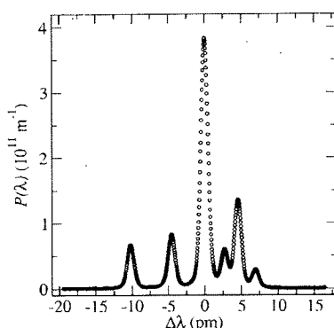
FIG. 4. Line profile function of the 2p_{10} \rightarrow 1s_5 transition in Xe obtained at
