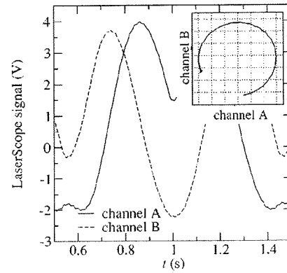
FIG. 2. Typical LaserScope signals; main frame: channels in y(t) mode with 90^\circ phase shift, inlay: same signals in xy mode. The laser is tuned over 0.8 \times \text{FSR} of the etalon.
