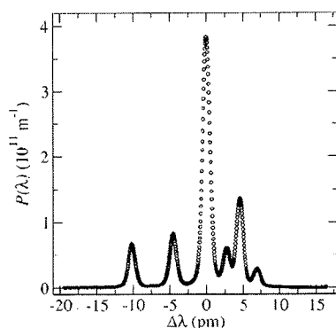
FIG. 4. Line profile function of the 2p_{10} \rightarrow 1s_{5} transition in Xe obtained at
