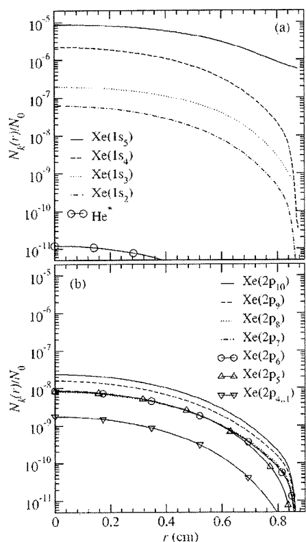
FIG. 6. Radial variation of the densities N_k of excited xenon and helium atoms for I_z=60 mA, p_0=2.5 Torr, and r_w=0.87 cm.
