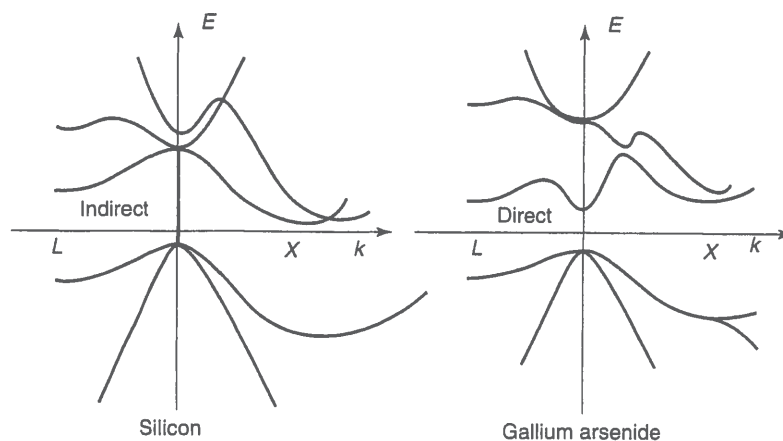
Figure 12.31 The distinction between a direct and indirect semiconductor material is often explained using the E (energy) versus k (momentum) diagram for the semiconductor. If the minima of the conduction band and the maxima of the valence band both occur at k = 0 , then the semiconductor is direct. If the minima and maxima do not overlap at all, or overlap at k \neq 0 , then the semiconductor is indirect.
