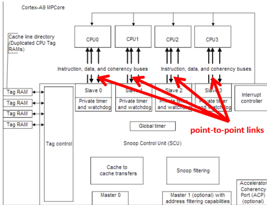
See Figure 1.1 of the Cortex-A9 Reference Manual (annotations added in red).
