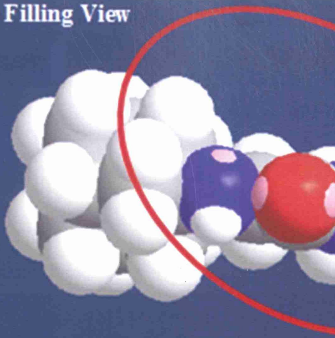
N-linked adamantyl
