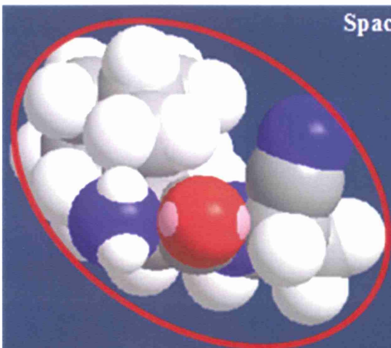
C-linked adamantyl
