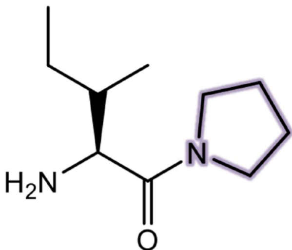
Compound 3 IC_{50} = 21 \mu M Saturated
