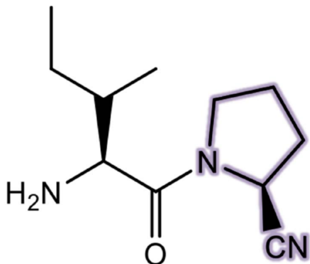
Compound 5 K_i = 2.2 \text{ nM} \pm 0.50
