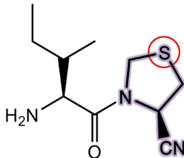
Compound 3 K_i = 0.41 \text{ nM} \pm 0.15
