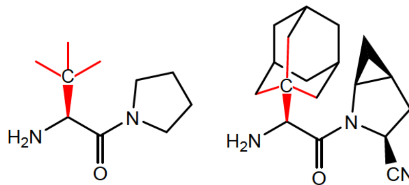
“Quaternary” beta-carbon
