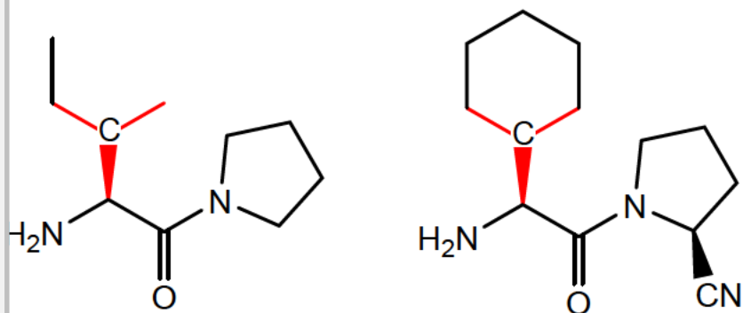
“Tertiary” beta-carbon
