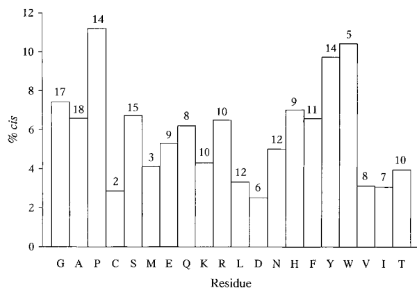
Figure 2. Histogram showing the percentage of occurrence of various residues in the cis conformation of the X-Pro peptide bond; the numbers of cis cases are given on top of each bar.
