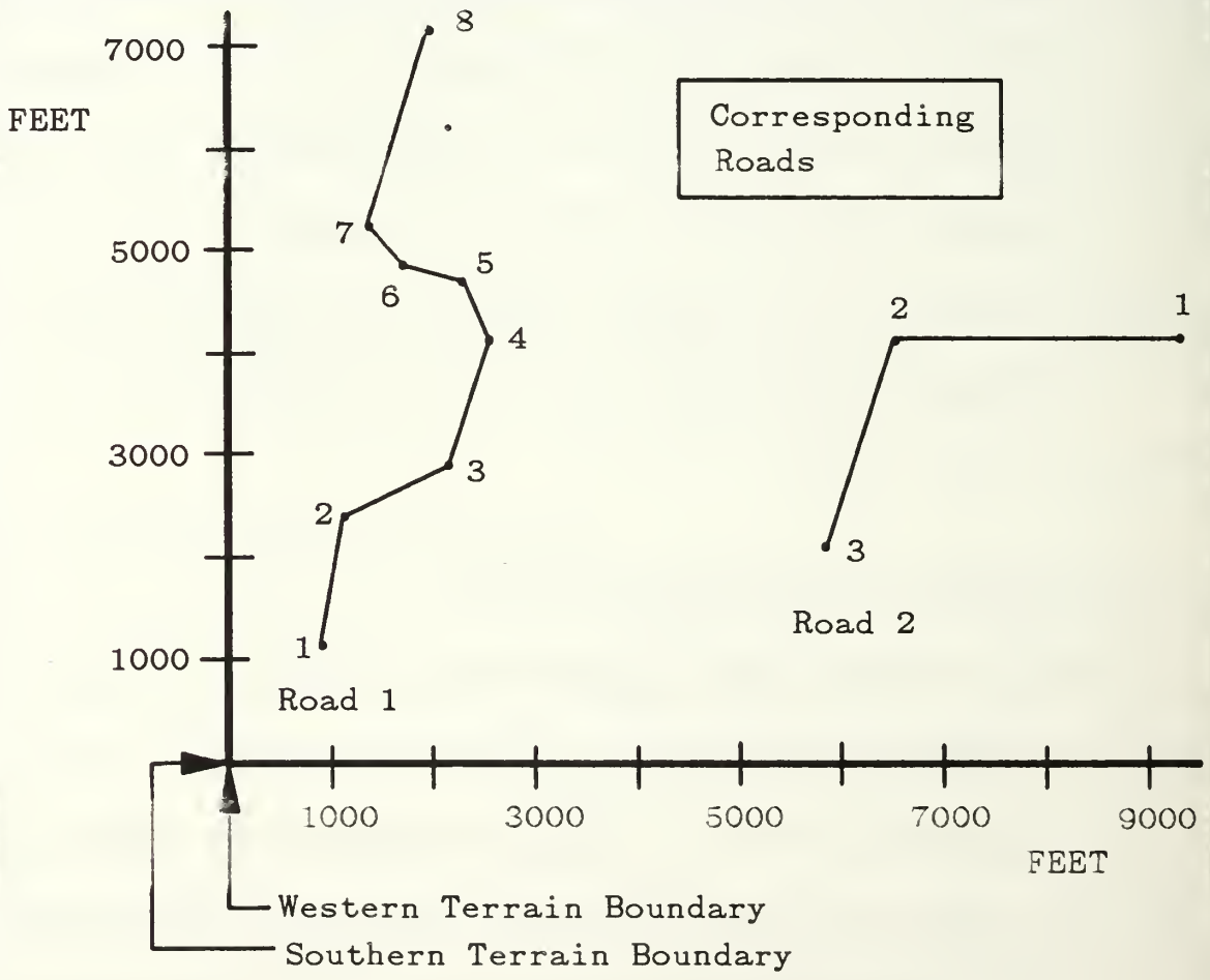
Figure 8.1 External Data File Format
