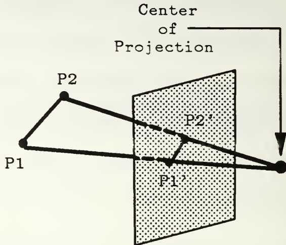
Perspective Projection
