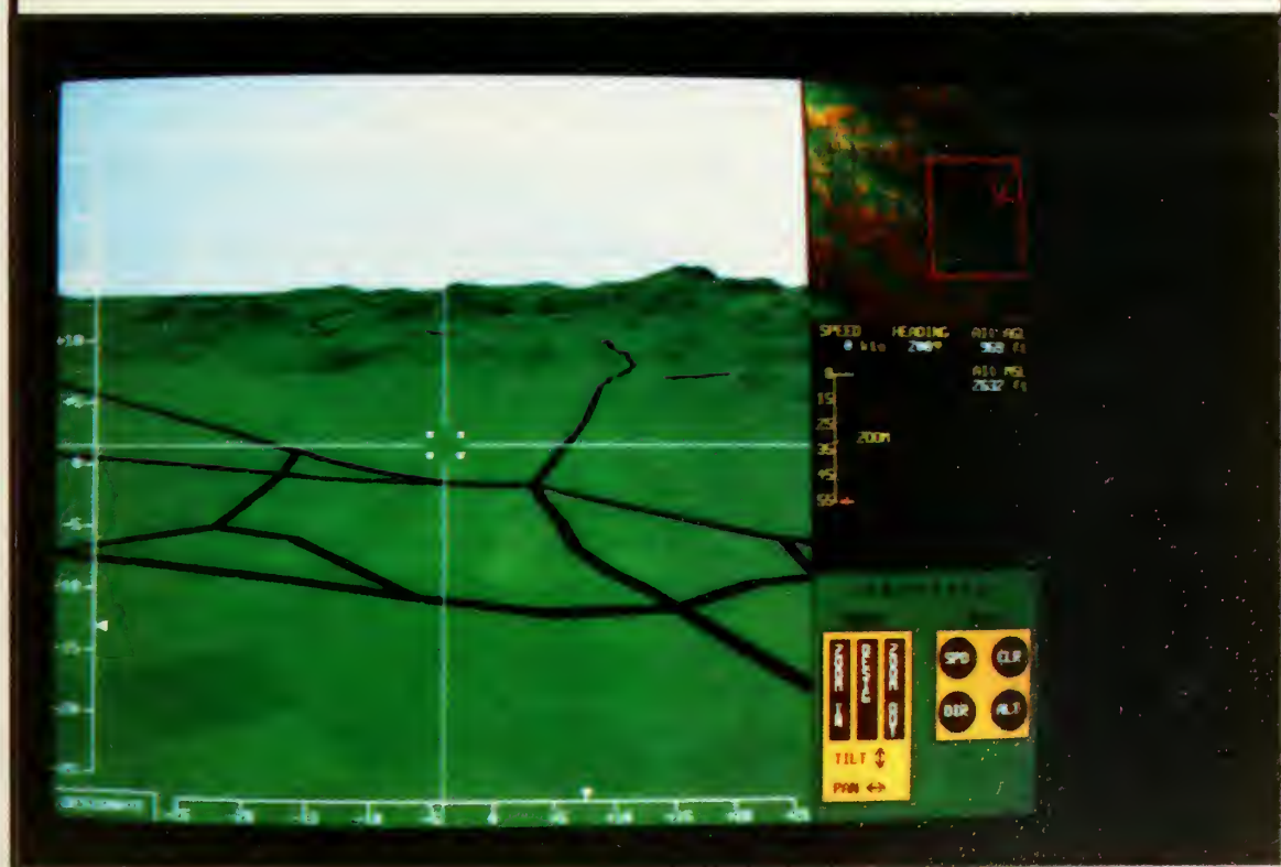
Figure 7.1 Simulator Scenes
