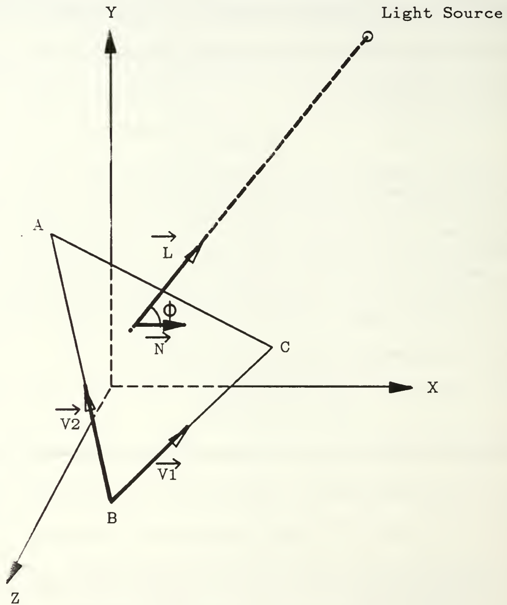
Figure 5.2 Lambert's Cosine Law
