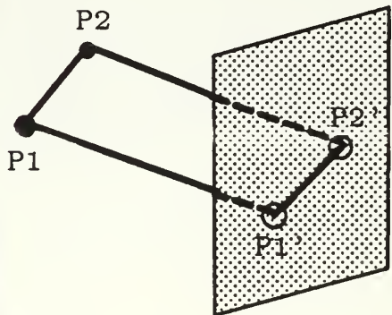
Parallel Projection
