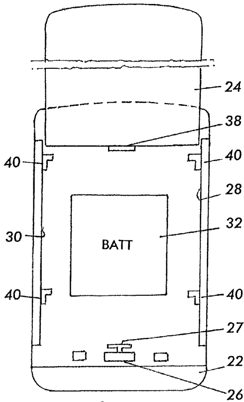
FIG. 2 (PRIOR ART)
