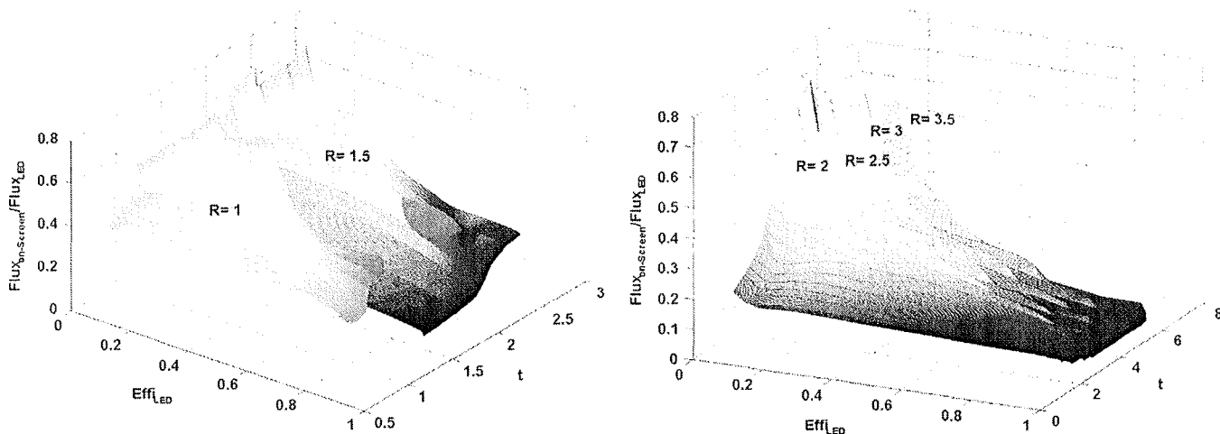
Fig. 4. (\eta_{\text{LED}})/(\Omega_{\% \text{LED}} A_{\text{pack}})\Omega_L A_L \eta_{\text{LE}} versus \eta_{\text{LED}} parameter space for the lens array.
