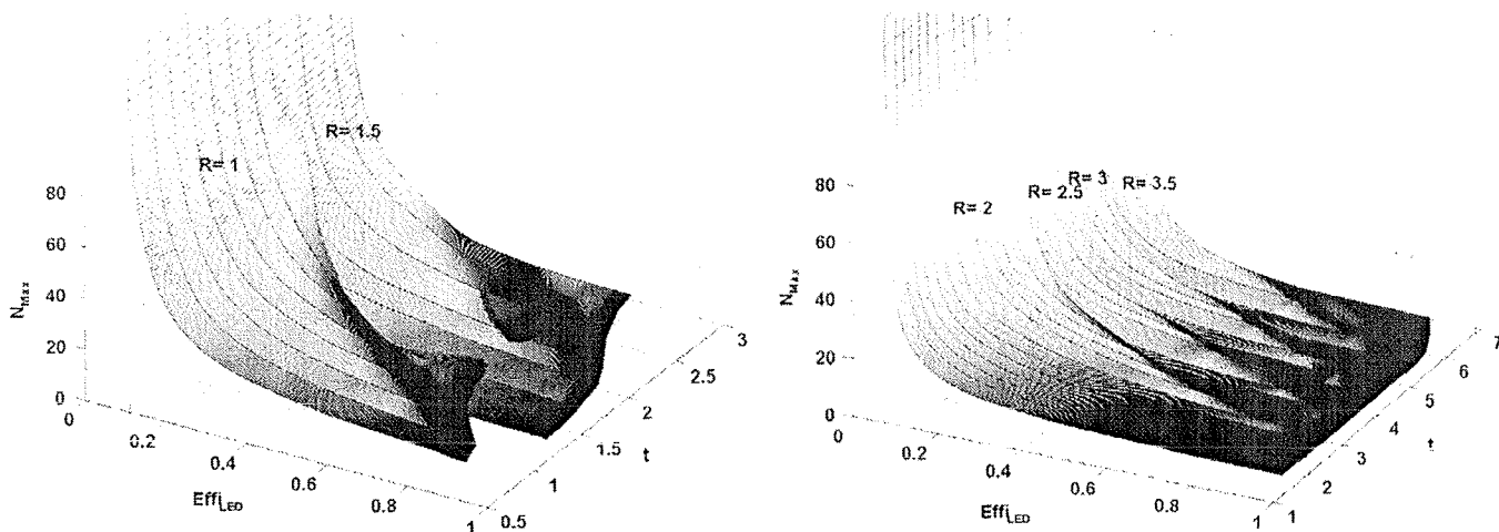
Fig. 5. Maximum LED number N versus \eta_{\text{LED}} parameter space for the lens array.
