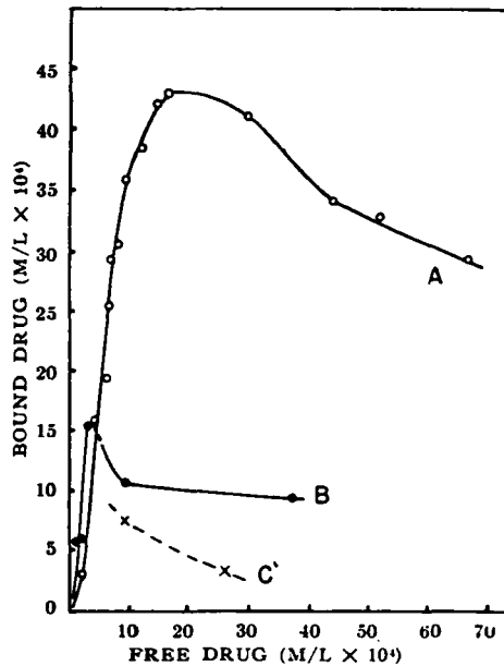
Fig. 6.—Adsorption isotherms for binding of cetylpyridinium chloride and cetyldimethylbenzylammonium chloride in 0.2% Tween 80 at 30°. These curves illustrate the degree of binding occurring at concentrations of the quaternary ammonium compounds both above and below their normal critical micelle concentrations. A, cetylpyridinium Cl; B, benzalkonium Cl(CDBAC); C, cetylpyridinium Cl, 0.05 M NaCl. Curve C illustrates the influence of electrolyte on the degree of interaction.
